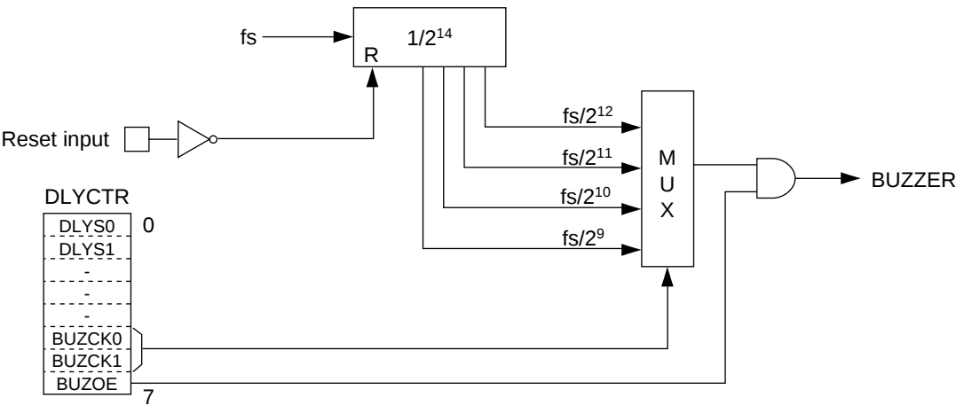
Figure 9-1-1 Block Diagram (Buzzer)
