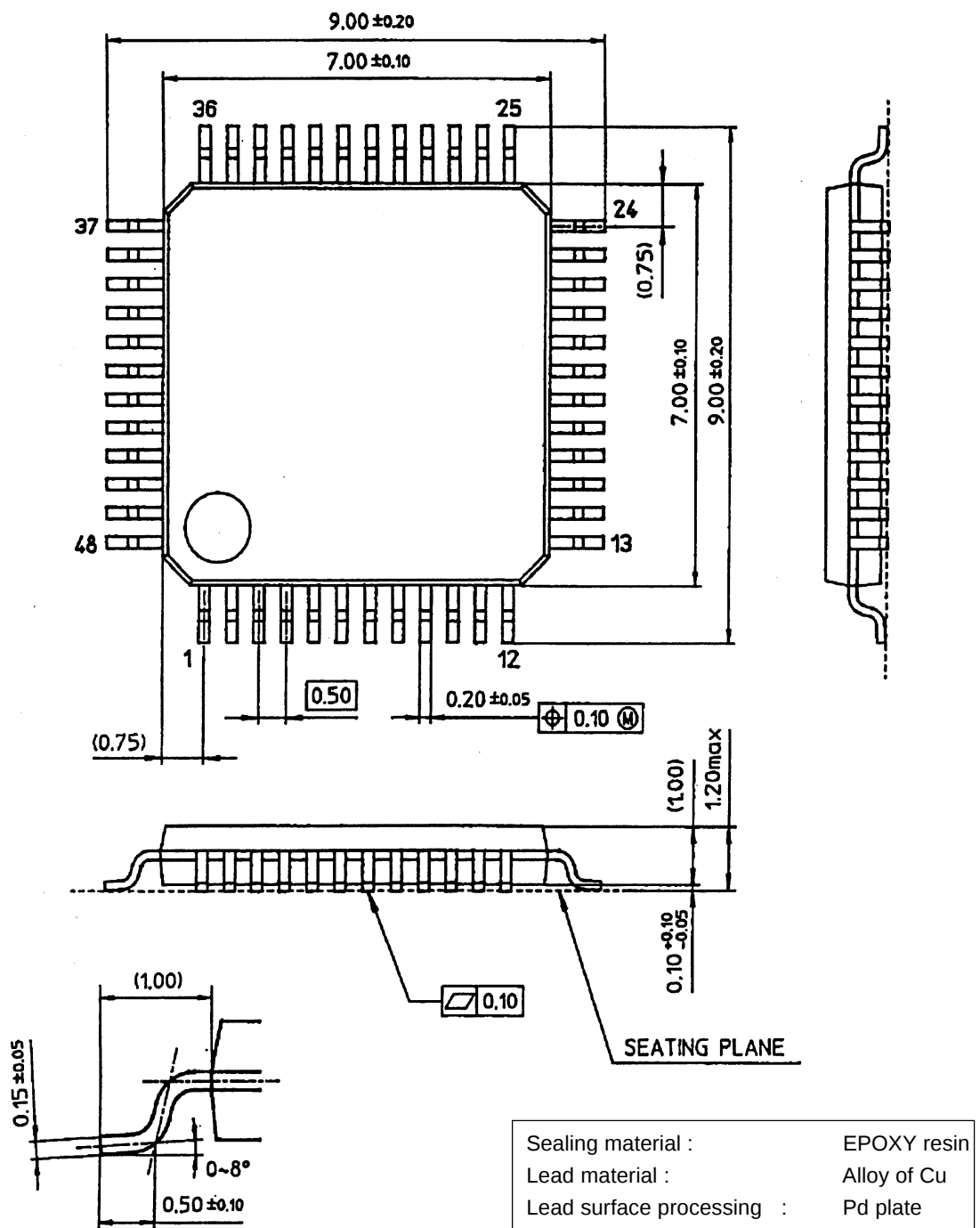
Figure 1-7-3 48-Pin TQFP
