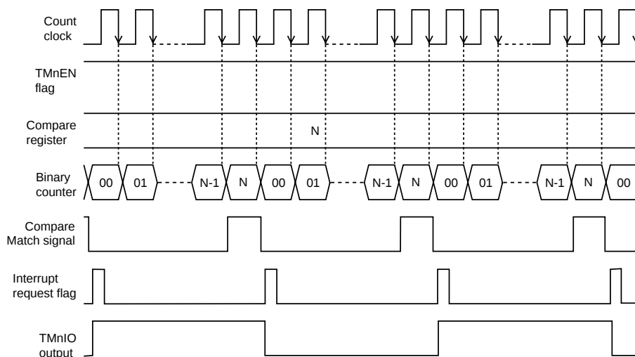
Figure 5-5-1 Count Timing of Timer Pulse Output (Timers 2 and 3)
