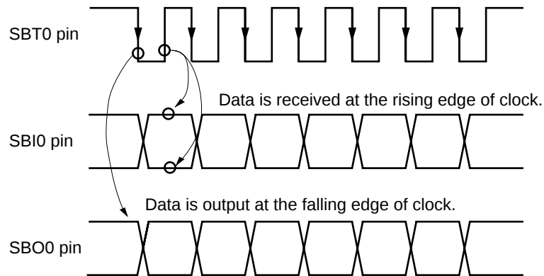
Figure 10-3-9 Transmission / Reception Timing (Reception : rising edge, Transmission : falling edge) (SC0CE0 = 0, SC0CE1 = 0)
