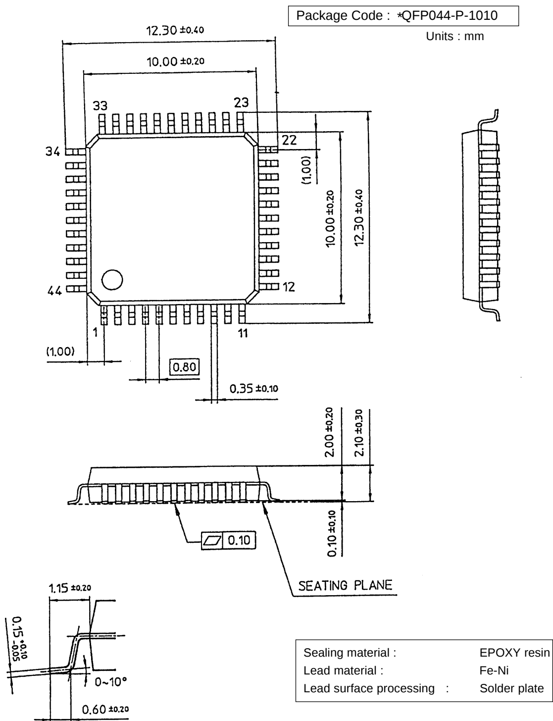
Figure 1-7-2 44-Pin QFP
