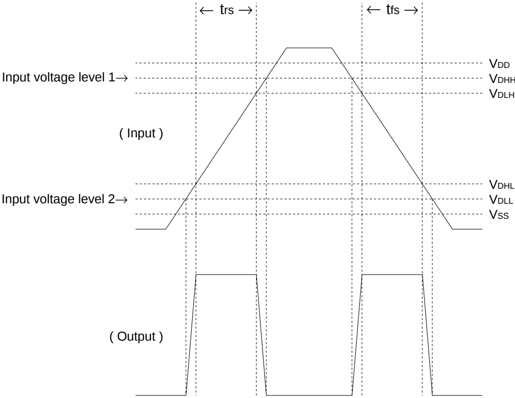
Figure 1-5-5 AC Zero-Cross Detector
