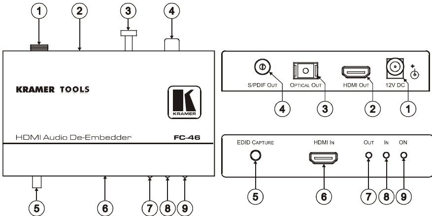
Figure 1: FC-46 HDMI Audio De-Embedder
