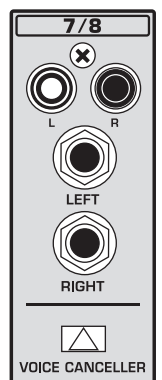
Fig. 3.2: Stereo channel connectors
