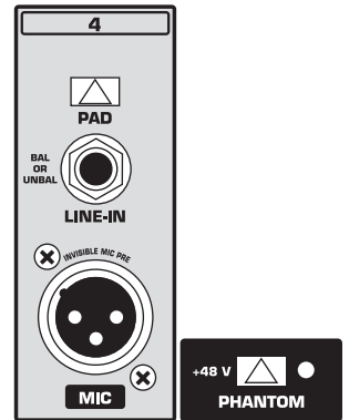
Fig. 3.1: Mono channel connectors
