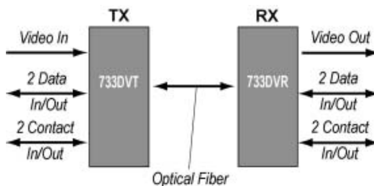
Figure 1. S733DV System Diagram
