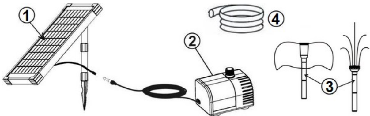
1)Solar panel with ground spike 2)Pump 3)Nozzles 4)Water hose
