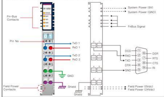
ST-5252 : 2Channels Serial Interface RS 232
