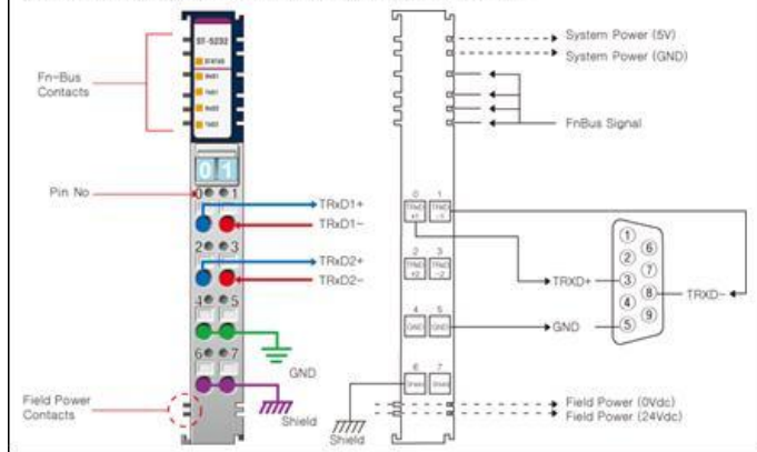
ST-5272 : 2Channels Serial Interface RS 485
