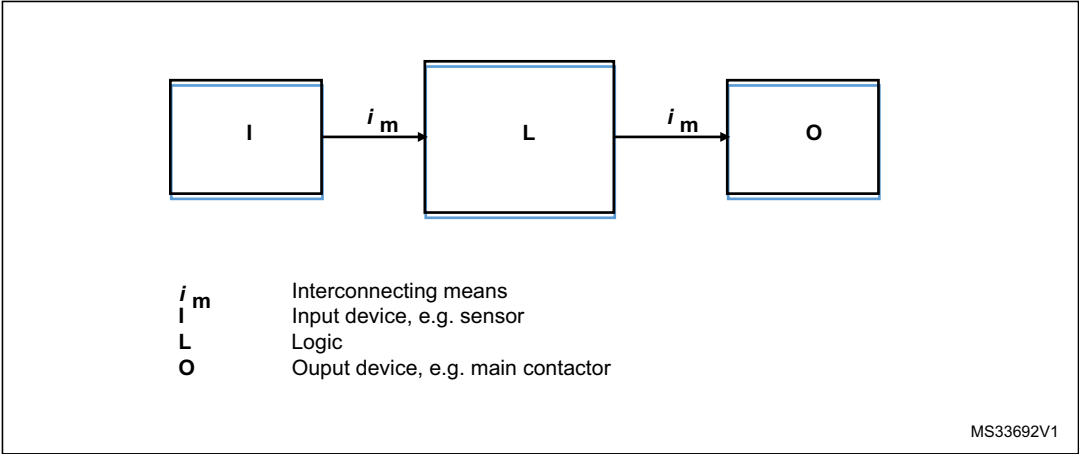
Figure 12. Block diagram for IEC 13849 Cat. B and Cat. 1
