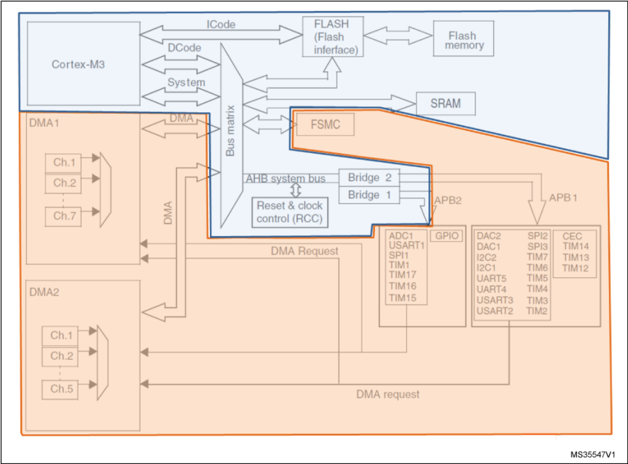
Figure 5. Block diagram of safety characteristics for STM32F1 modules
