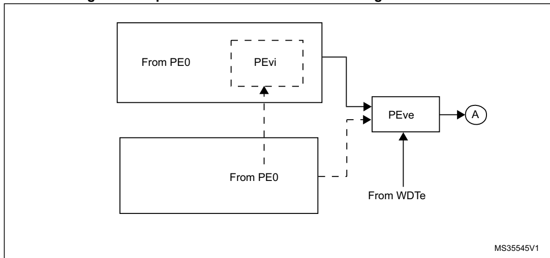
Figure 11. A possible voter structure combining PEvi and PEve
