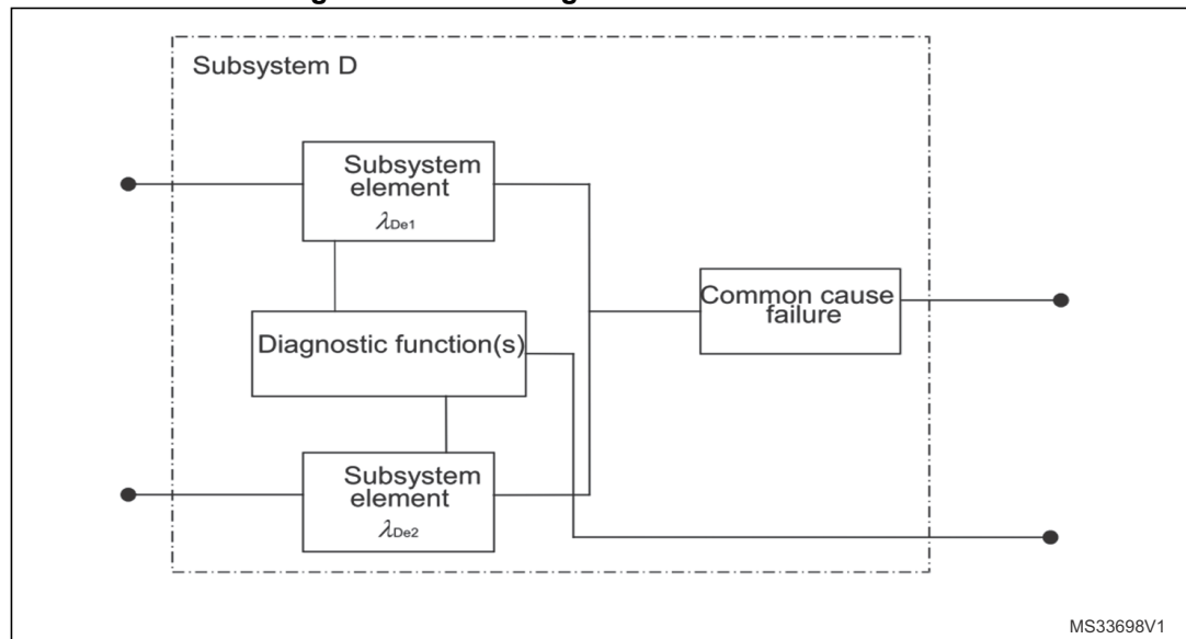
Figure 18. Block diagram for IEC 62061 Cat. D
