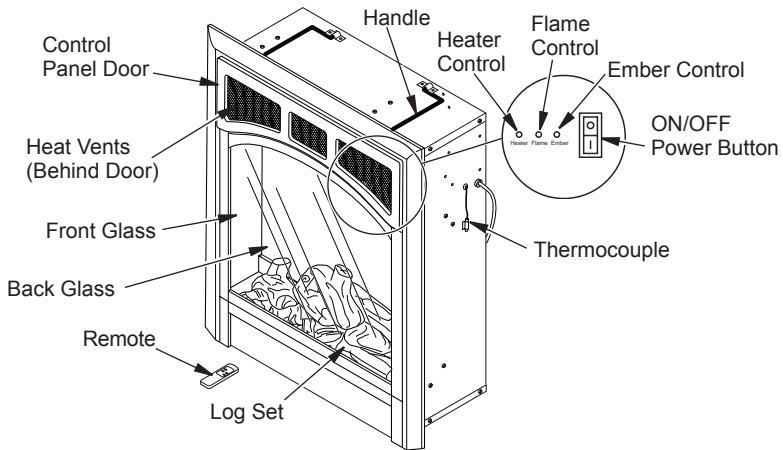
Figure 2 - Product Identification
