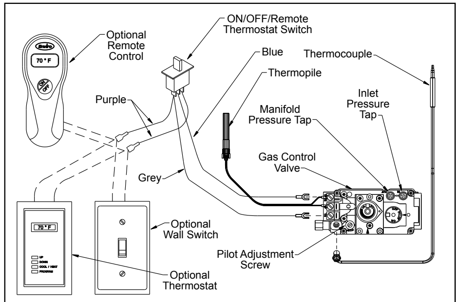
Figure 51: Gas Control Valve and Optional Thermostat Wiring.
