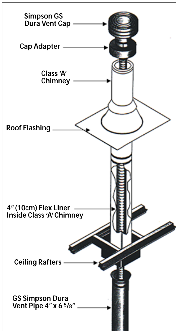
Figure 39: Assembly of Venting into a Class 'A' Chimney.
