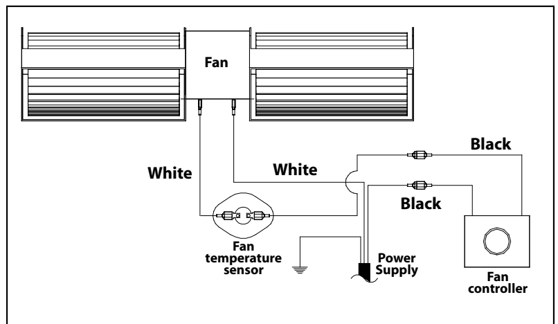
Figure 52: Wiring Diagram For Fan Control.
