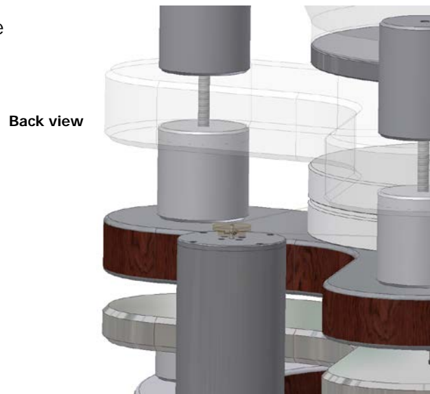
Pic. 21: Placing the drive belt
