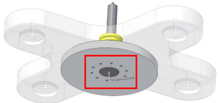
Pic. 15: To attach the upper drive platter to the bottom of the main bearing spindle
