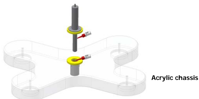
Pic. 13: Oiling the main bearing spindle
