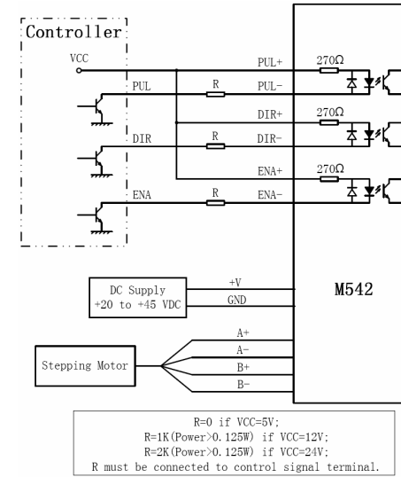
Figure 10: Typical connection
