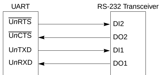
Figure 30-2. UART/RS-232 Interface
