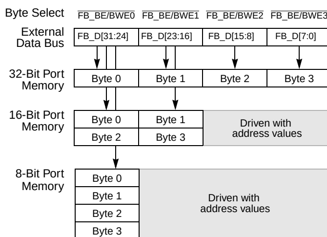
Figure 17-4. Connections for External Memory Port Sizes ( \text{CSCR}_n[\text{SBM}] = 0 )
