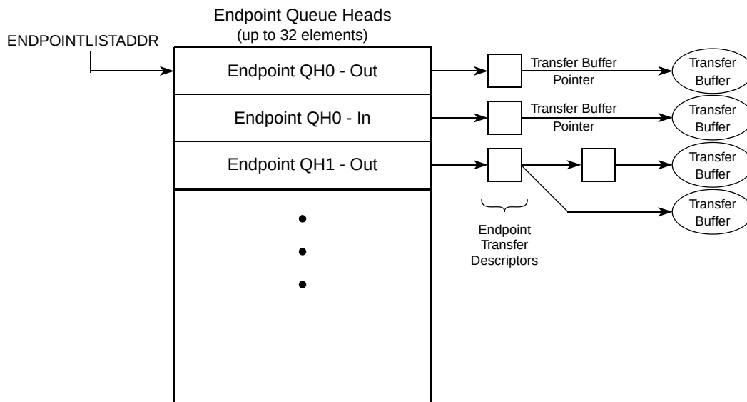
Figure 21-40. Endpoint Queue Head Diagram
