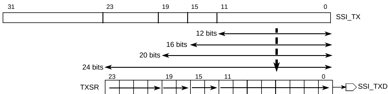
Figure 23-8. Transmit Data Path (TXBIT0=1, TSHFD=1) (lsb Alignment)
