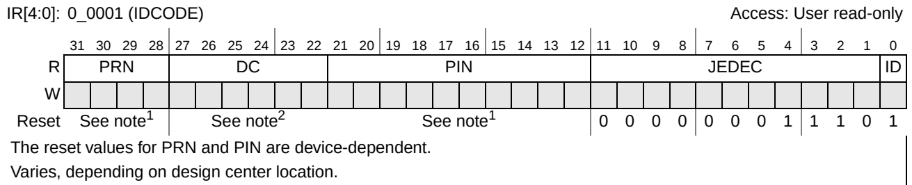
Figure 36-3. IDCODE Register
