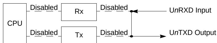
Figure 30-23. Remote Loopback
