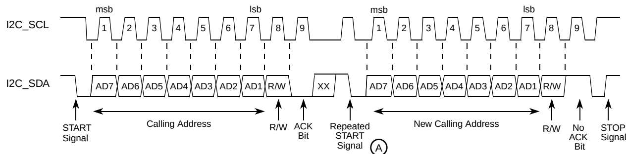
Figure 31-10. Repeated START
