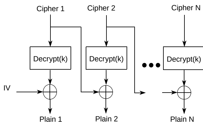
Figure 34-6. CBC Decryption
