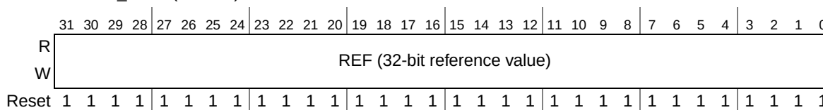
Figure 28-5. DTRRn Registers
