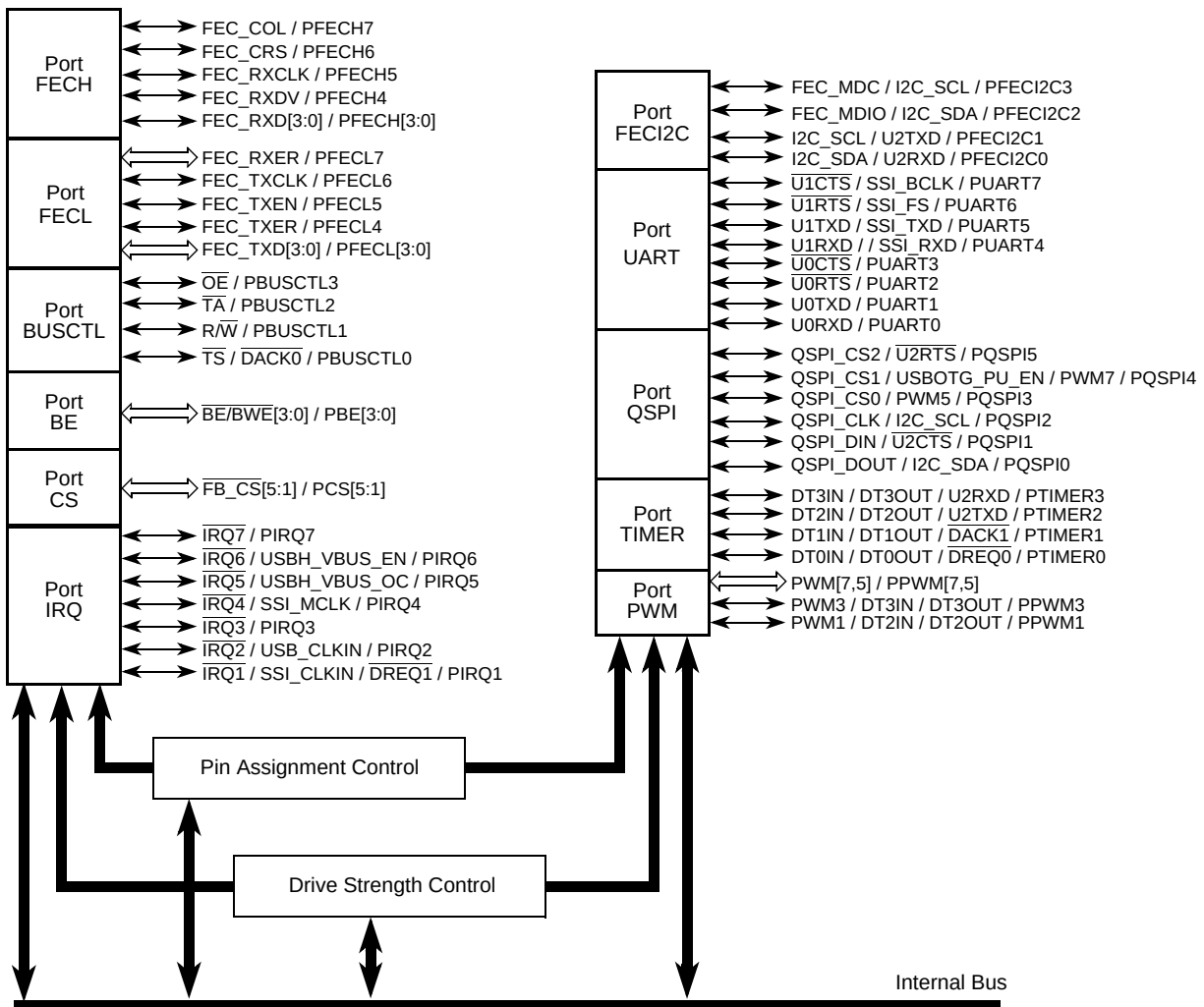
Figure 13-1. Ports Module Block Diagram
