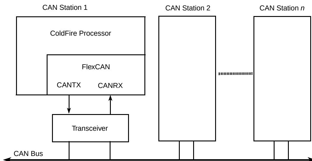
Figure 22-3. Typical CAN System
