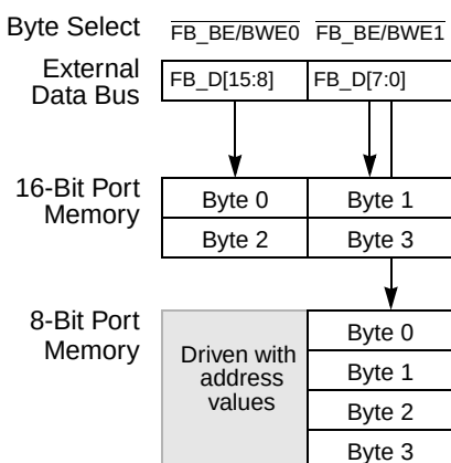
Figure 17-5. Connections for External Memory Port Sizes ( \text{CSCR}_n[\text{SBM}] = 1 )
