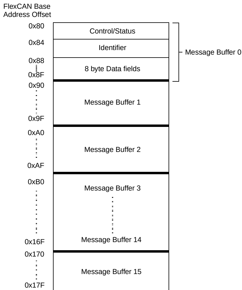
Figure 22-12. FlexCAN Message Buffer Memory Map
