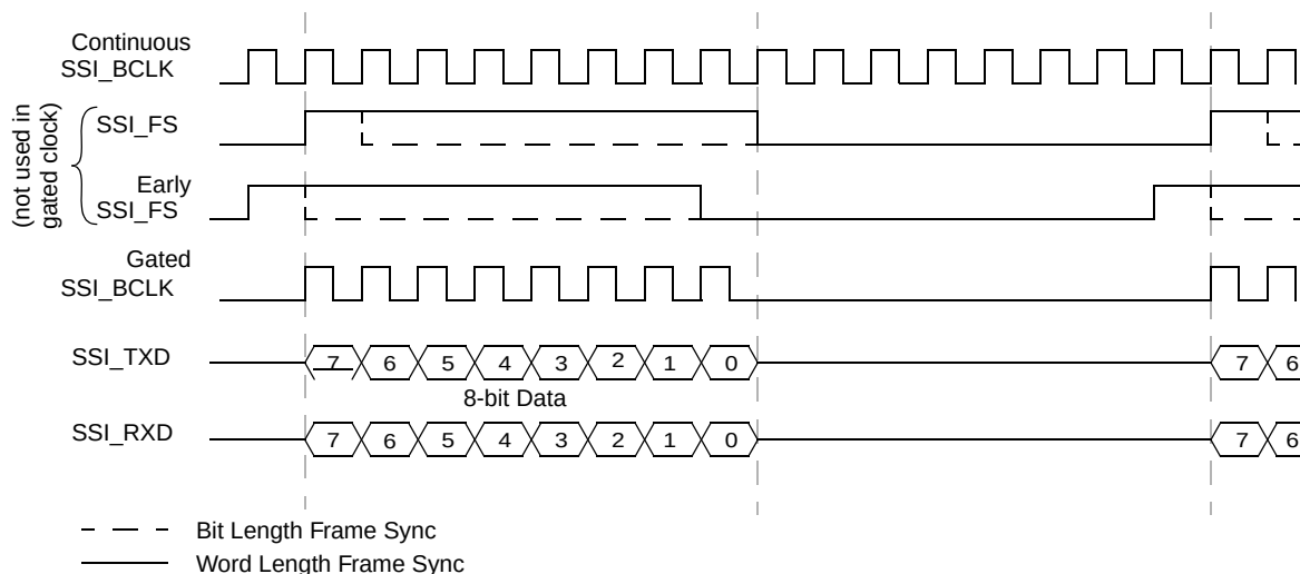
Figure 23-3. Serial Clock and Frame Sync Timing
