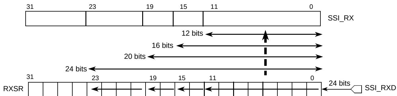
Figure 23-12. Receive Data Path (RXBIT0=1, RSHFD=0) (lsb Alignment)
