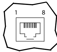
RJ45 Connector (Back of unit)
