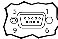
Female DB9 Connector (Back of unit)
