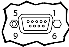
Female DB9 Connector (Back of unit)
