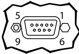
Female DB9 Connector (Back of unit)
