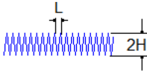
Figure 4. Dimensions of the satin outline/appliqué stitch. "H" (height) is the half height (for satin and bean stitches) and "L" (length) is the stitch-to-stitch running length.
