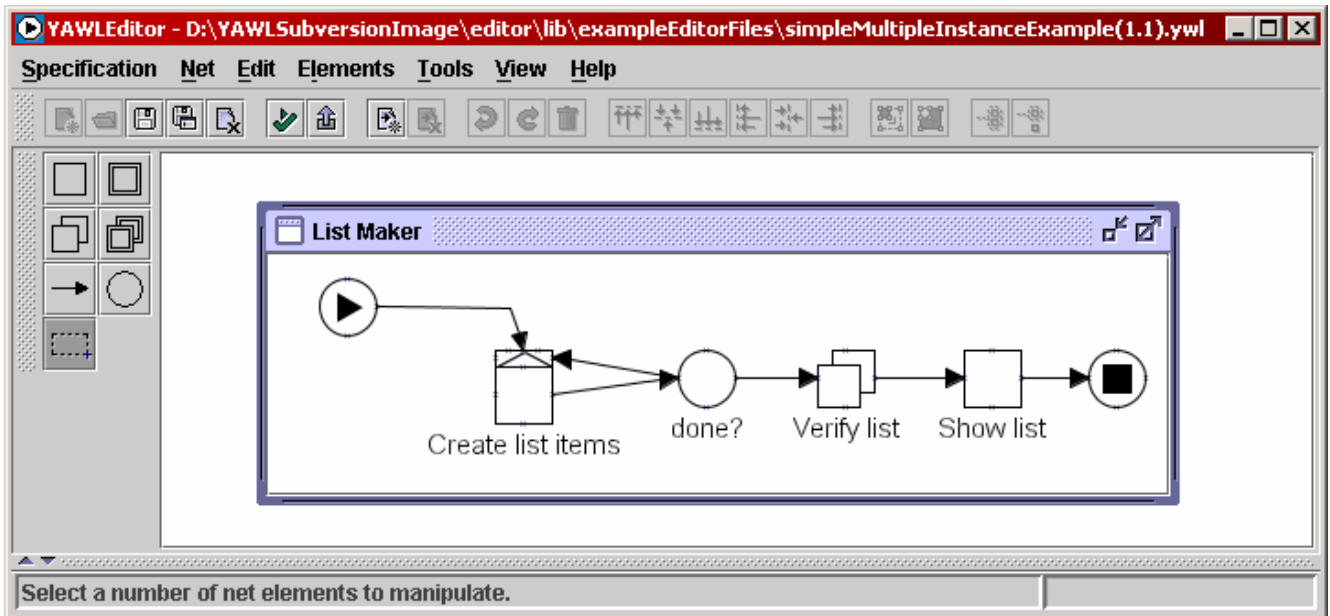
Fig. 40 - A simple specification showing how multiple instance tasks are done.
