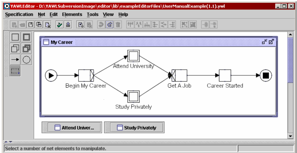
Fig. 14 - Making the "Study Privately " task atomic
