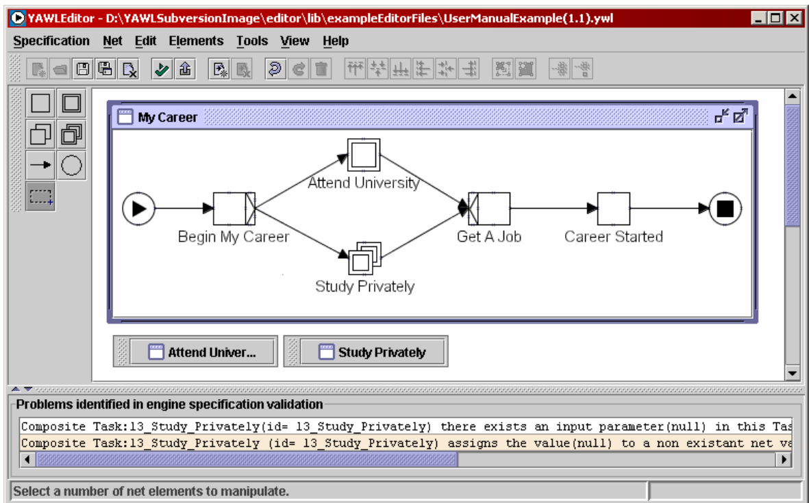
Fig. 13 - Validation with unfinished Multiple-Instance Tasks
