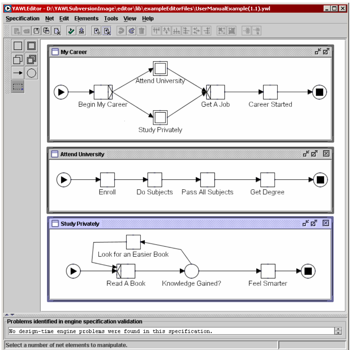
Fig. 33 - The completed scenario specification
