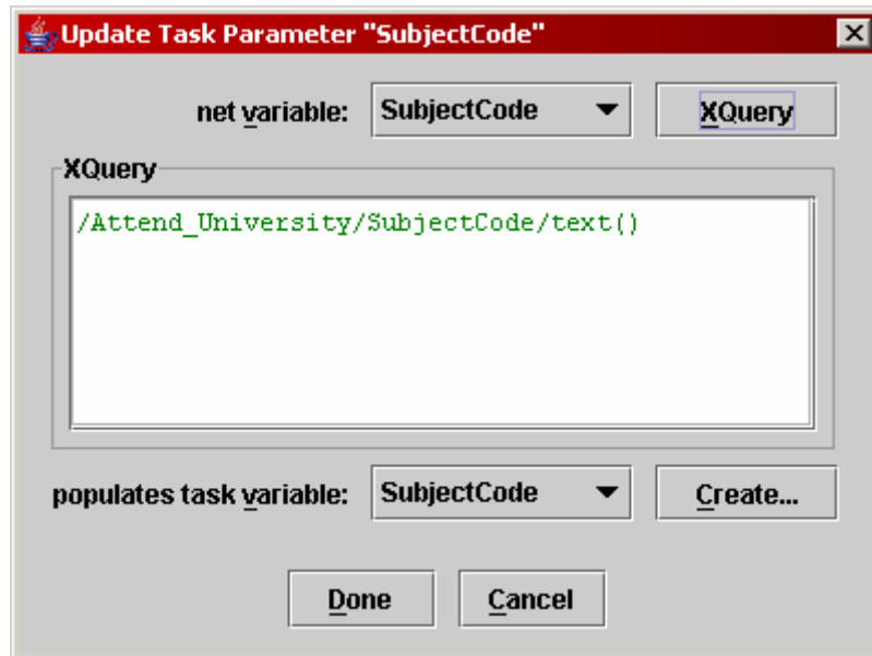
Fig. 30. Passing a net's SubjectCode to a Task
