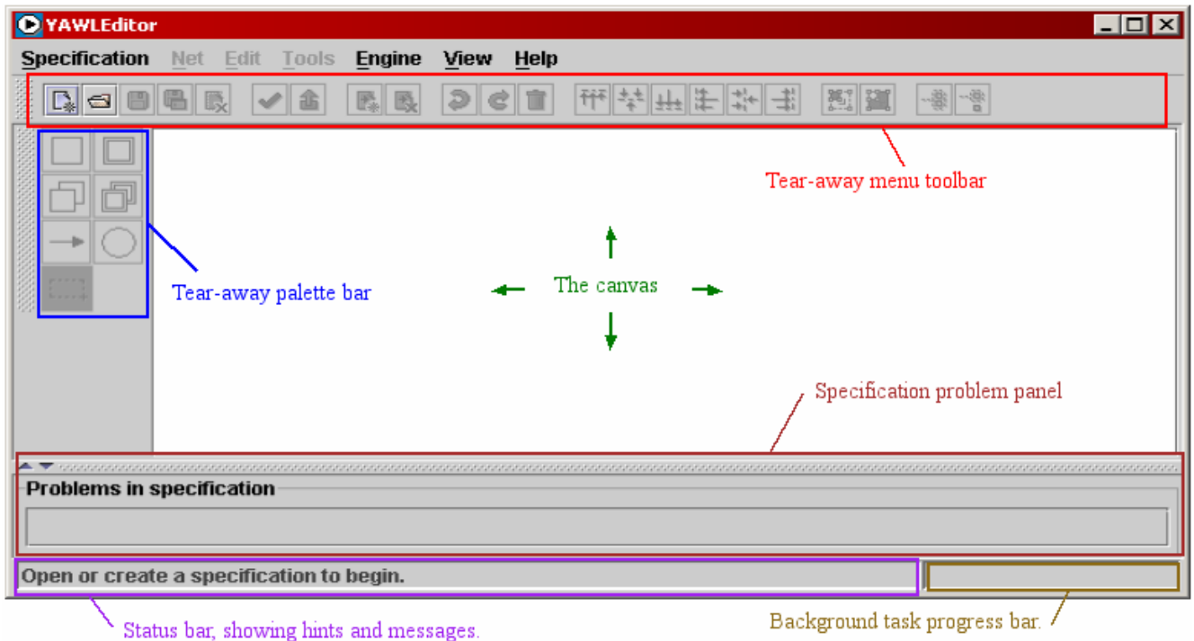
Fig. 2. The YAWL Editor Workspace
