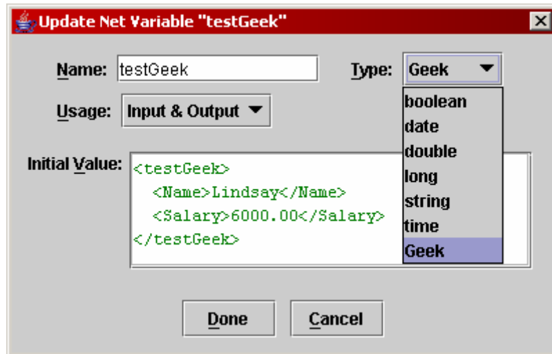
Fig. 21. A "Geek" task variable
