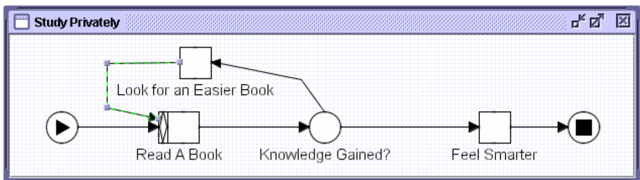
Fig. 16. Adding “knees” to a Flow Relation
