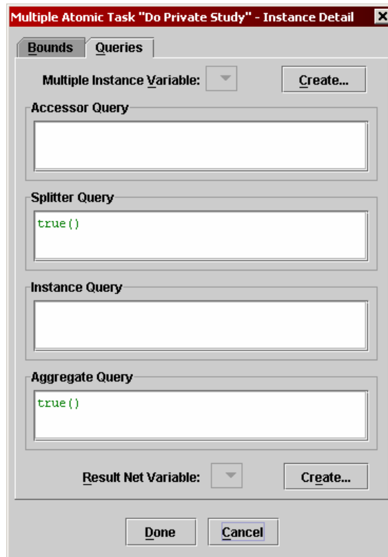
Fig. 35. Data Manipulation for Multiple Instance Tasks
