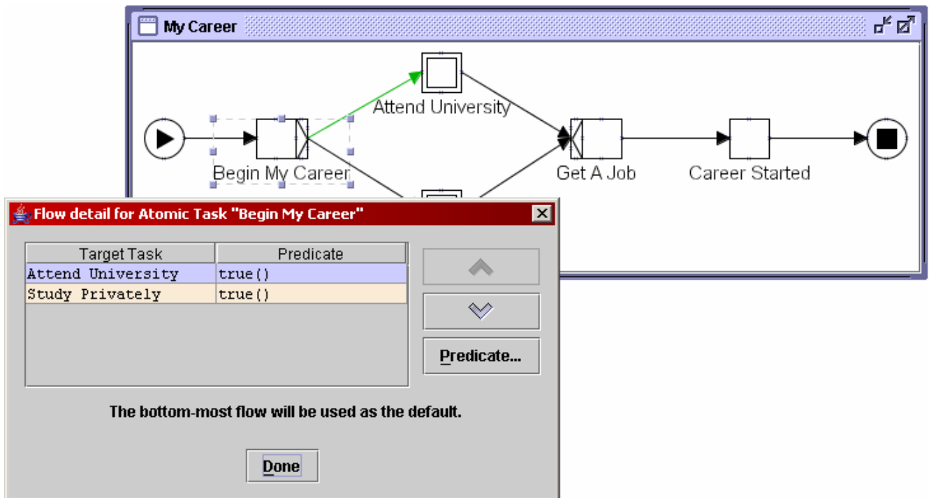
Fig. 32. Updating the Flow Detail
