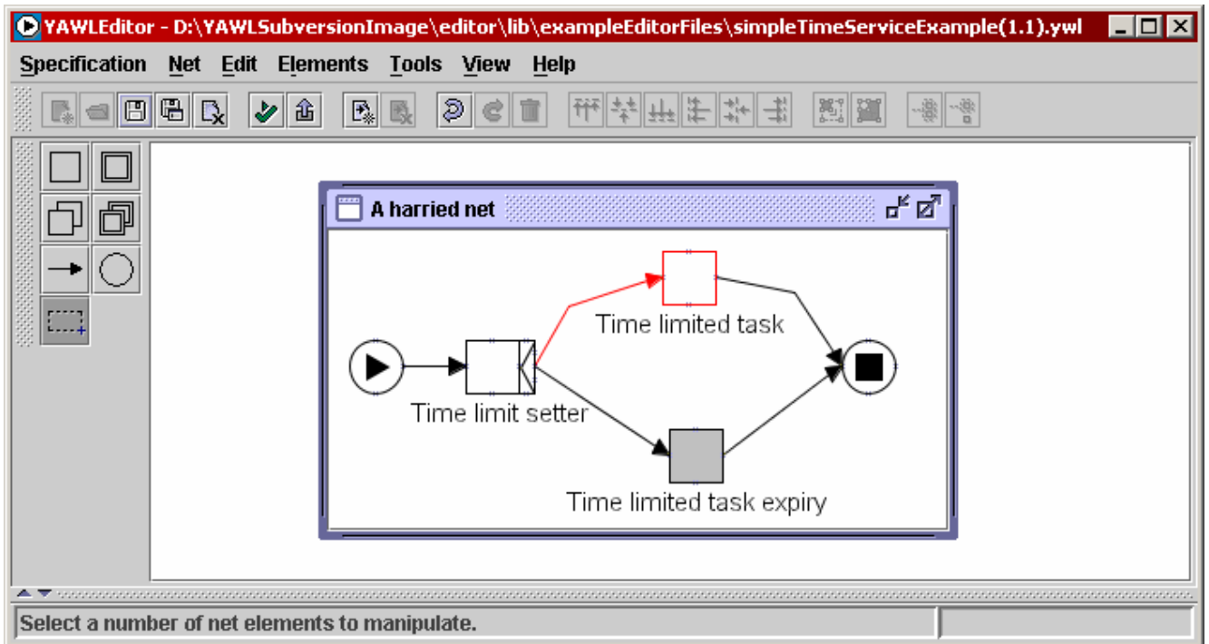
Fig. 43 - Example showing the usage of a custom YAWL service
