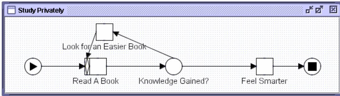
Fig. 12. Condition Loop for “Study Privately” Net
