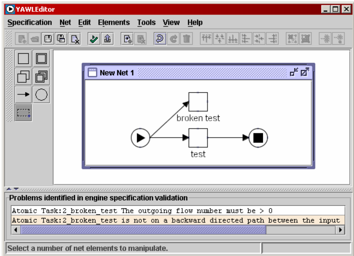
Fig. 37. An invalid specification
