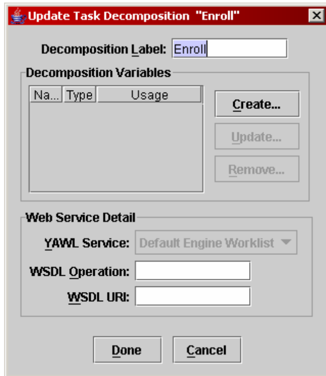
Fig. 26. Updating variables for a task
