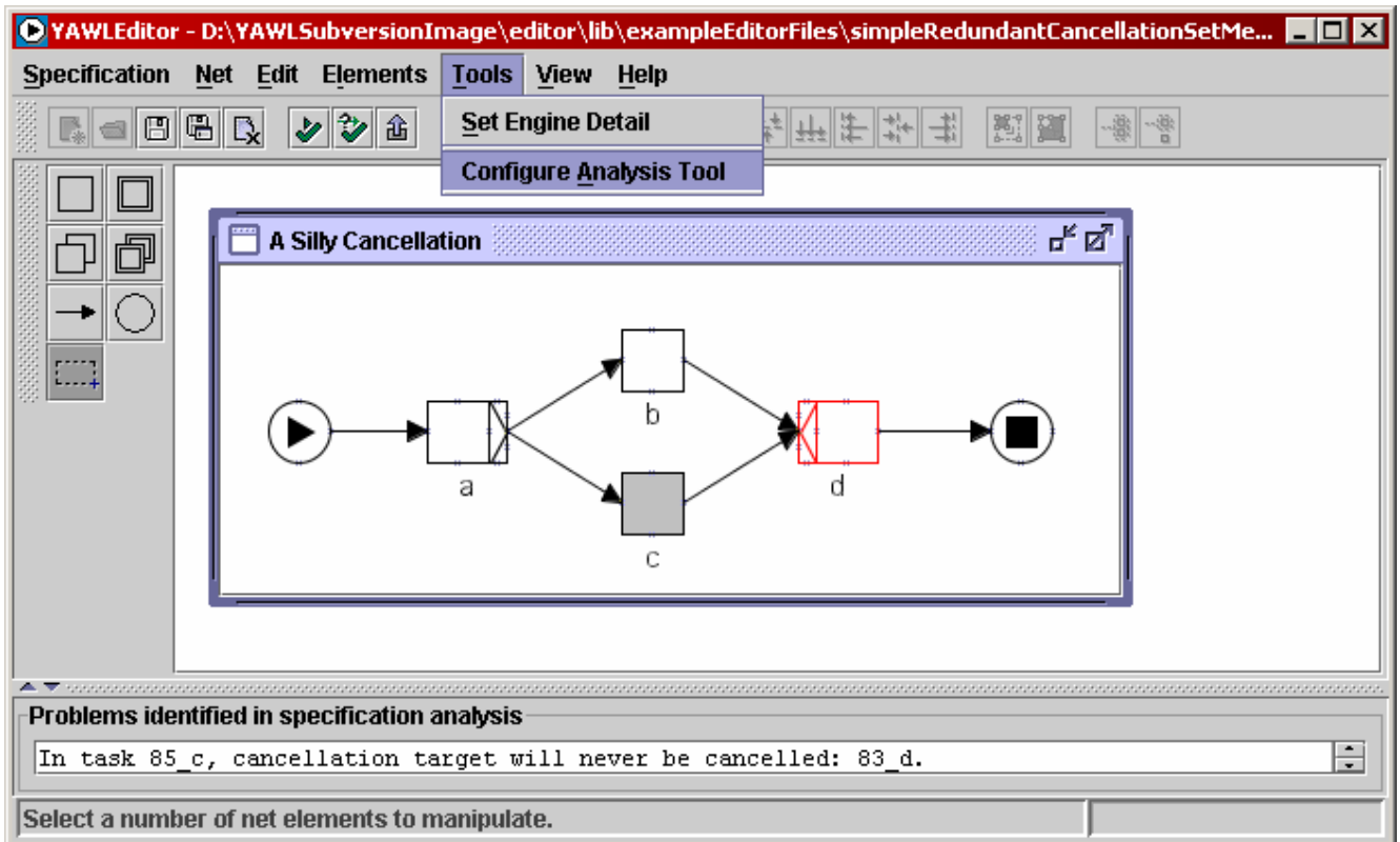
Fig. 38. Specification analysis functions
