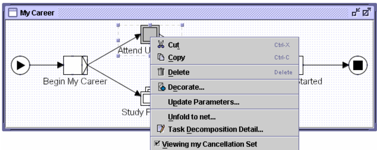
Fig. 18. Viewing a task's cancellation set
