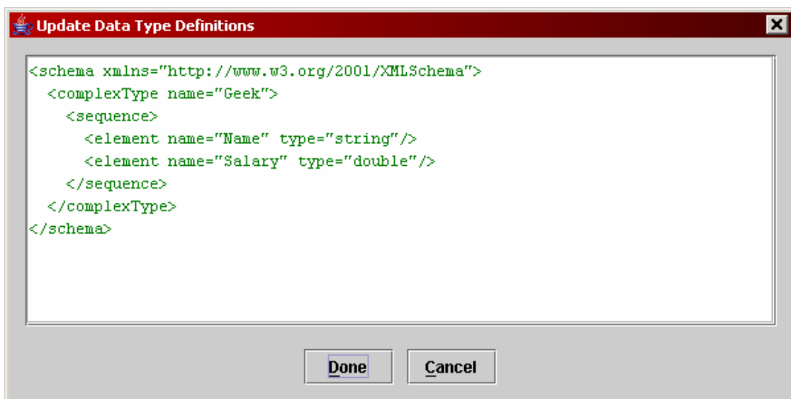
Fig. 20. Adding the "Geek" complex data type
