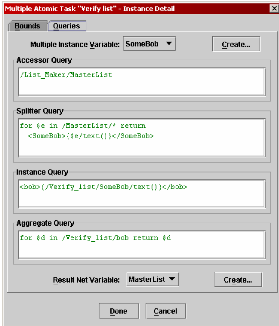
Fig. 42 – Example multiple instance queries
