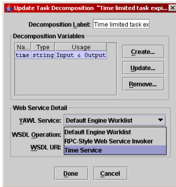
Fig. 44 - Assigning a registered YAWL service from a running engine
