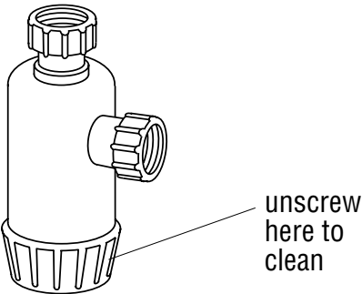
Bottle trap
