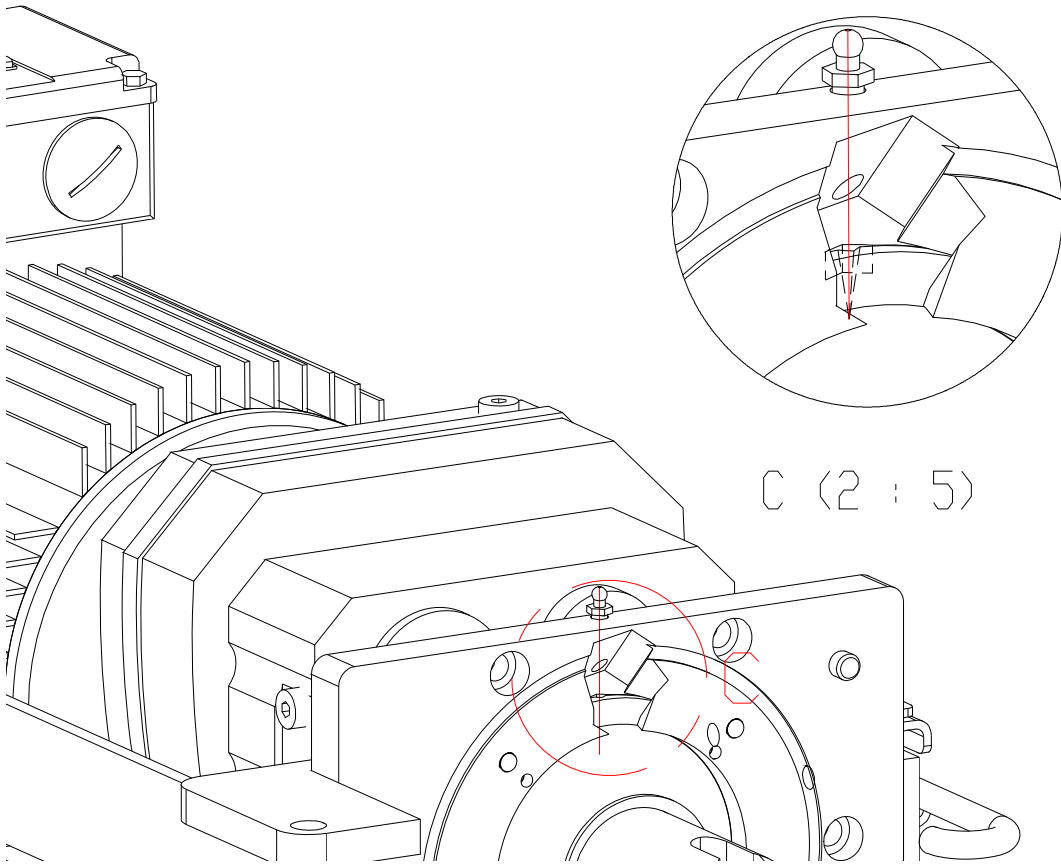
Showing relationship between grooves in adaptor and seal, to allow grease to flow
