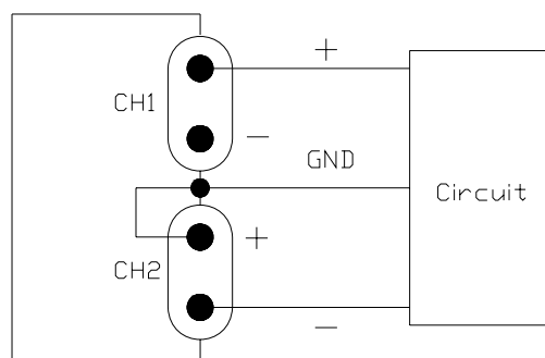
Regulated DC Power Supply Illustration of Bi-Polar Tracking Mode
