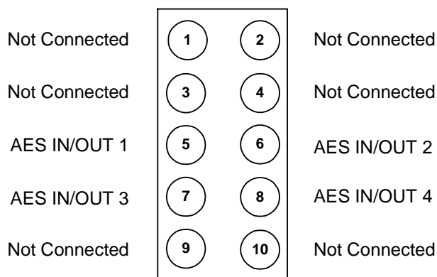
Figure 3. BNC Designations for the Card Rear Module 8310-RM-10 or 8310-RM-100
