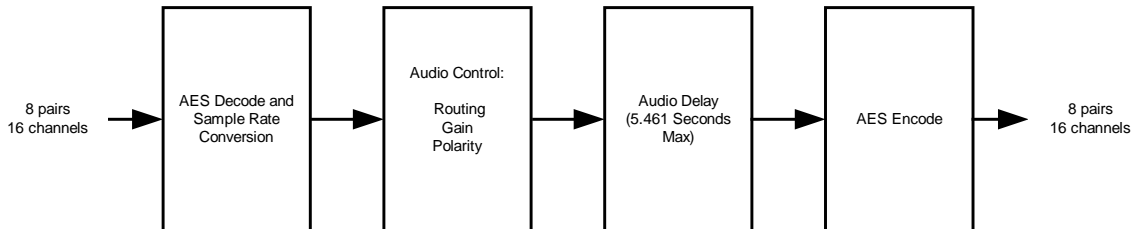
9301 Block Diagram
