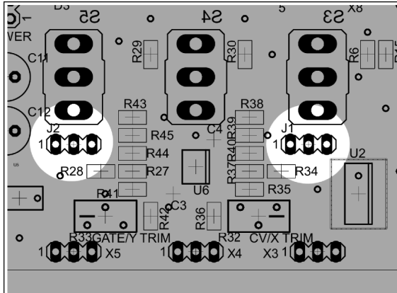
Output Offset Jumpers
