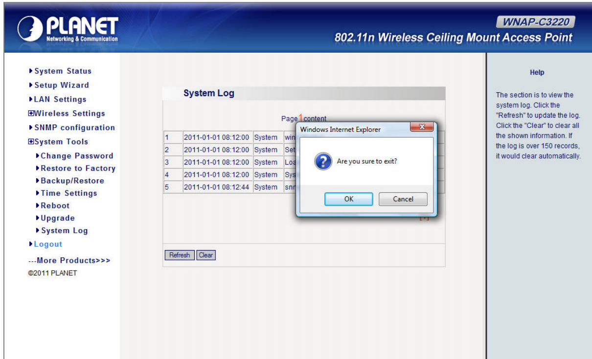
Figure 39 Logout
