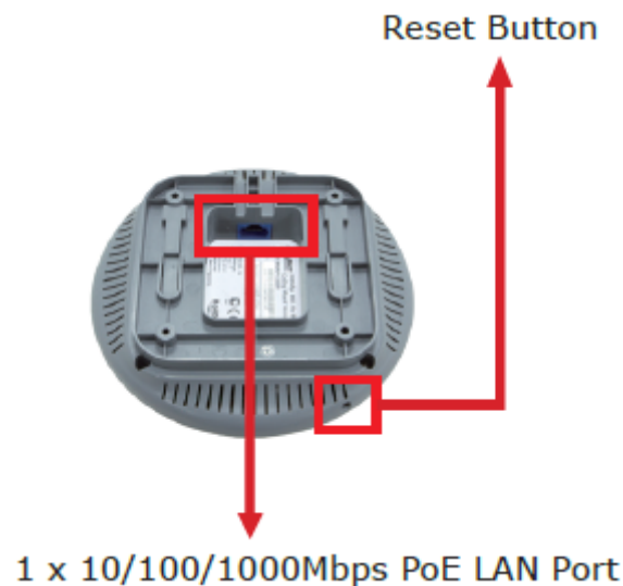
Figure 3 Rear Panel - 2
