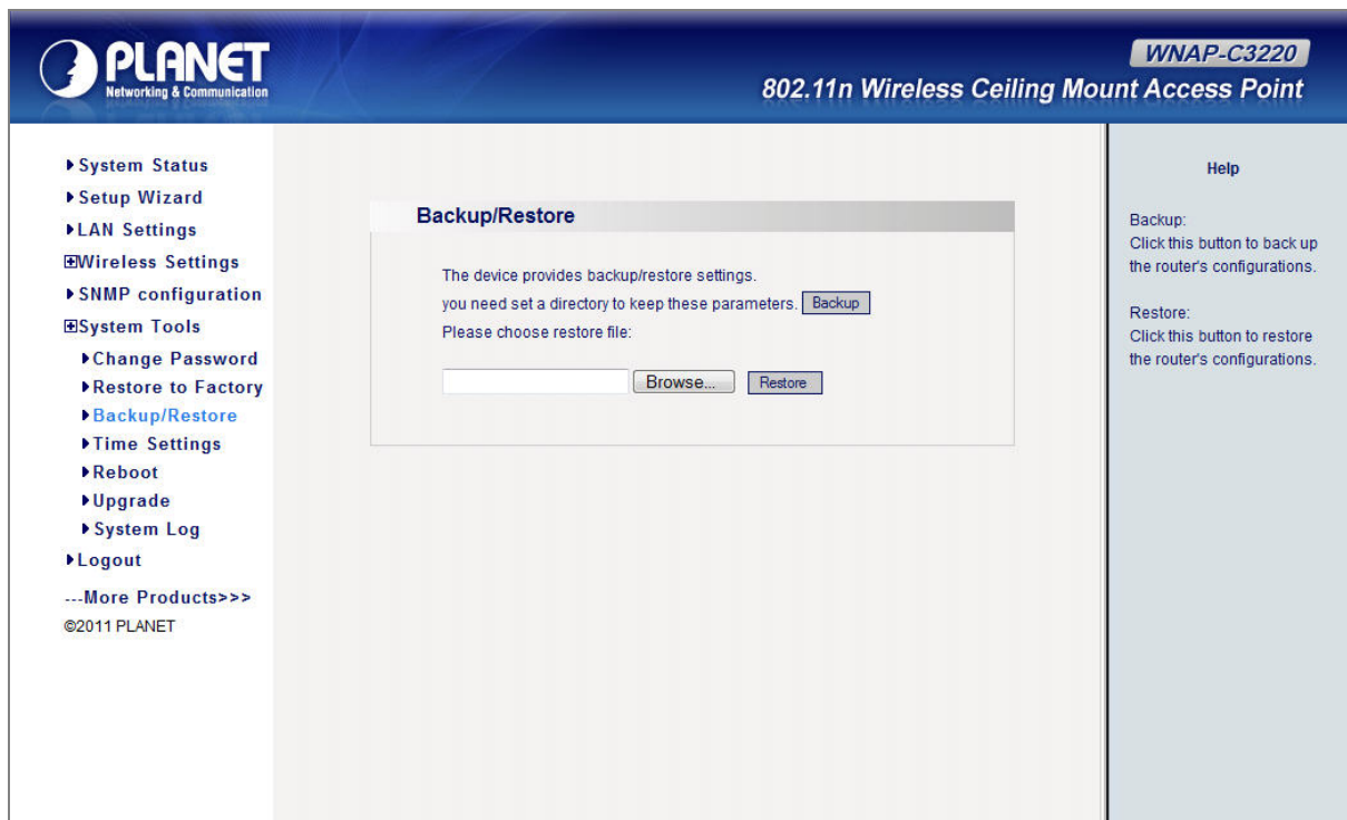
Figure 35 Backup/Restore
