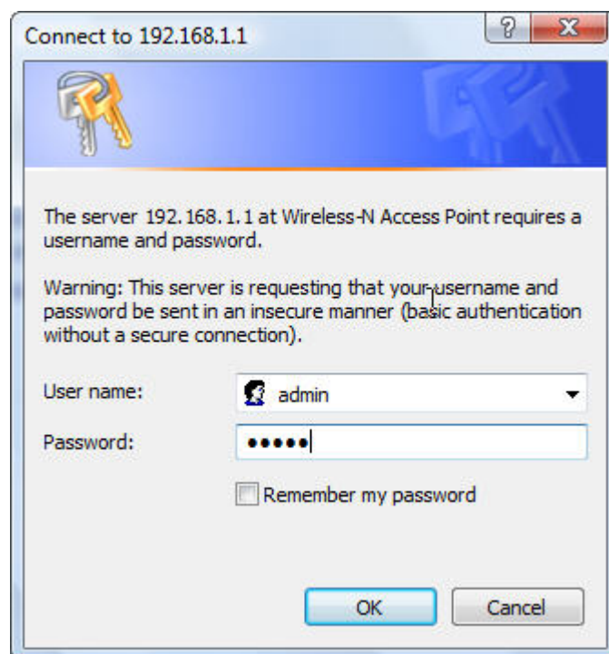
Figure 15 Login Window
