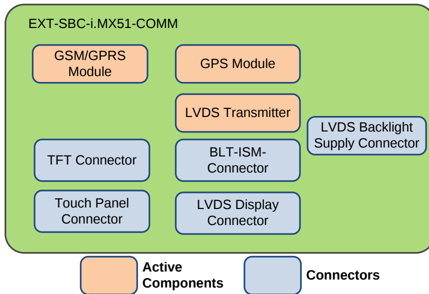
Figure 1-2: Main components of EXT-SBC-i.MX51-COMM
