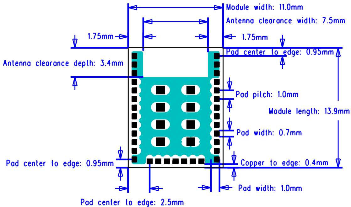
Figure 22 BT121 module physical dimensions
