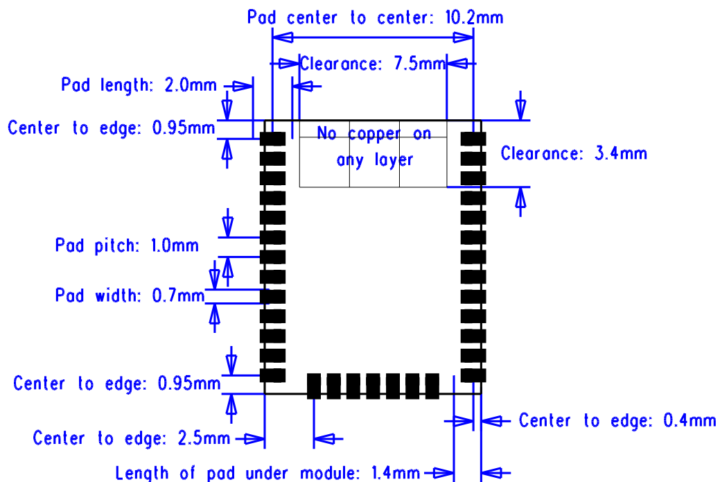
Figure 23 BT121 module recommended PCB pad pattern
