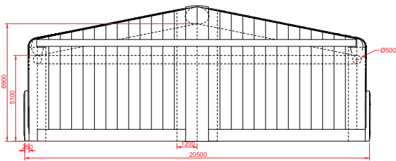
SIDE ELEVATION
