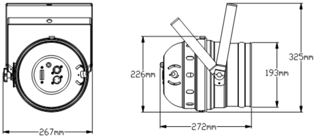
LED PAR64 (short can)
