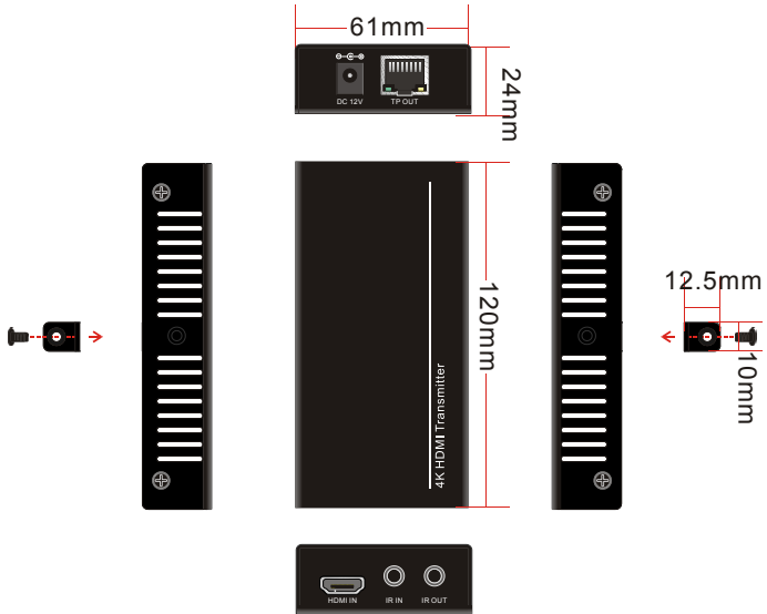
HDBaseT Transmitter
