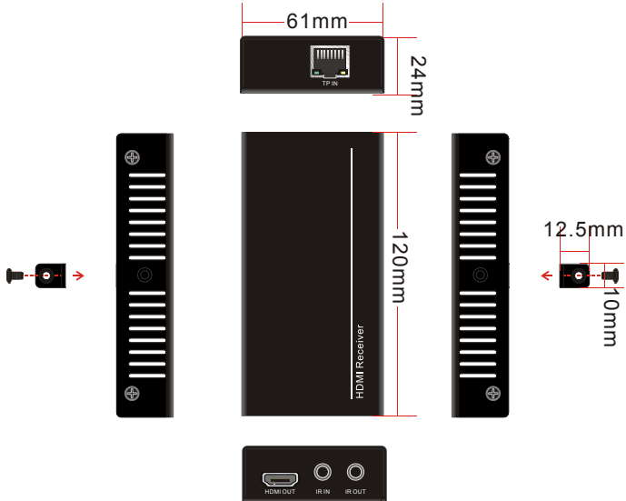
HDBaseT Receiver
