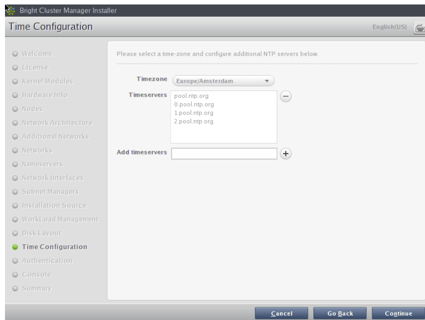
Figure 2.20: Time Configuration
