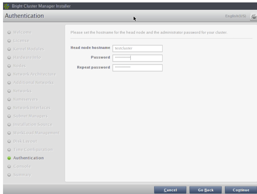
Figure 2.21: Authentication
