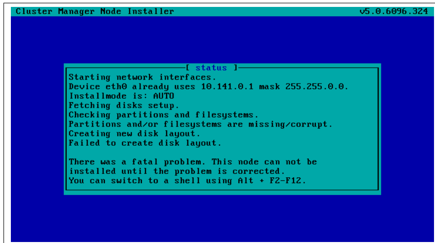
Figure 6.25: No Disk
