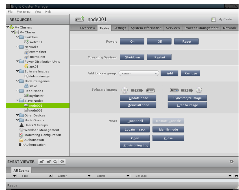
Figure 3.6: Node Tasks
