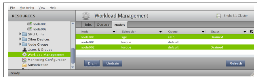
Figure 8.9: Node Drainage
