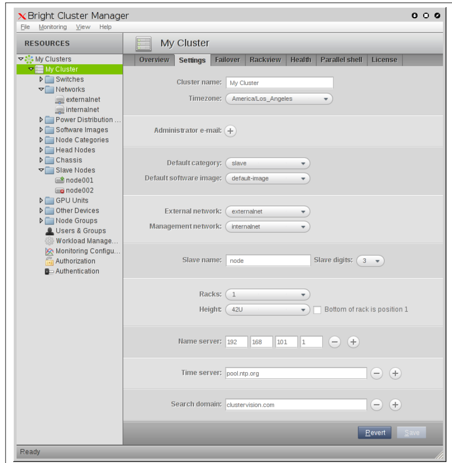
Figure 4.6: Cluster Settings
