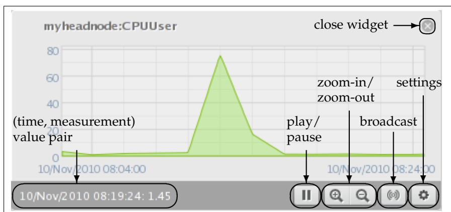
Figure 10.8: Graph Display Pane: Features
