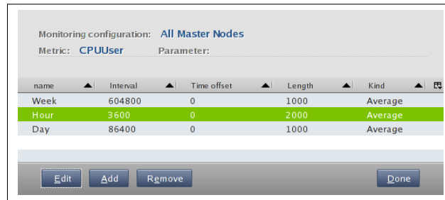
Figure 10.20: cmgui Metric Configuration: Consolidators Display
