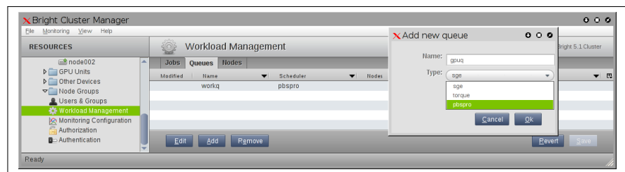
Figure 8.10: Adding A New Queue Via cmgui
