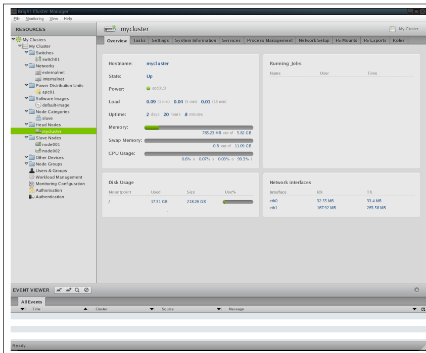
Figure 5.4: Head Node Overview
