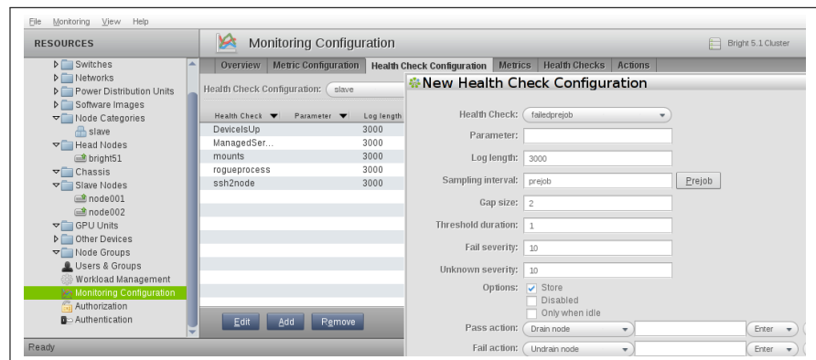
Figure 8.14: Configuring A Prejob Healthcheck Via cmgui
