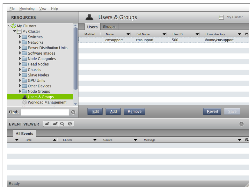
Figure 7.1: cmgui User Management
