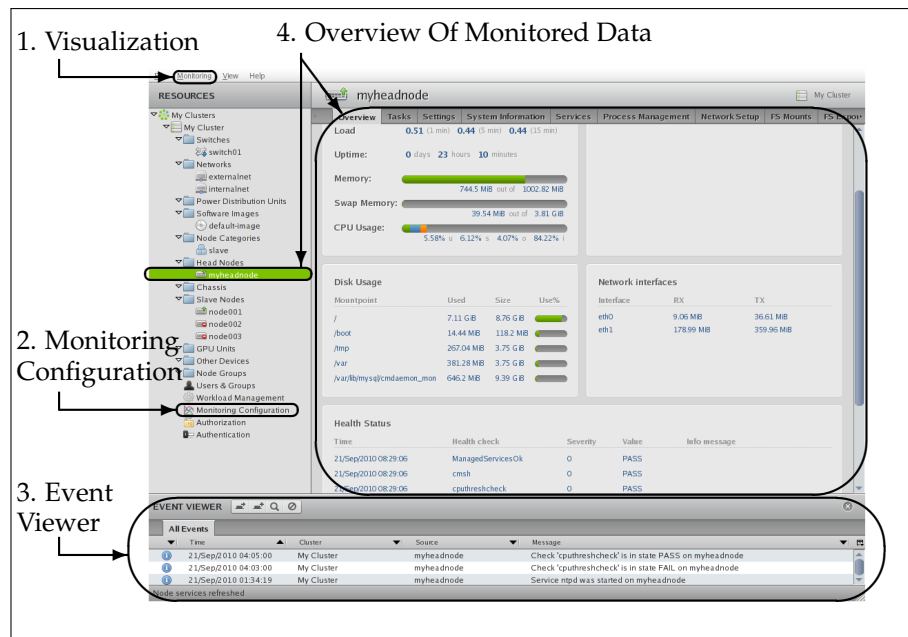
Figure 10.4: cmgui Conceptual Overview - Monitoring Types
