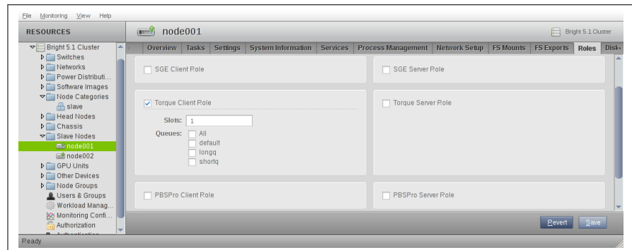
Figure 8.3: Workload Management Role Assignment For An Individual Node
