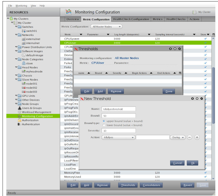
Figure 10.3: cmgui Monitoring Configuration: Setting A Threshold
