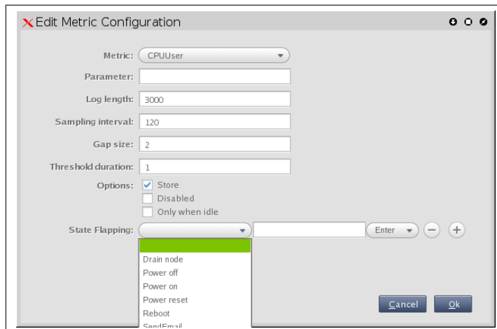
Figure 10.17: cmgui Monitoring: Metric Configuration Edit Dialog
