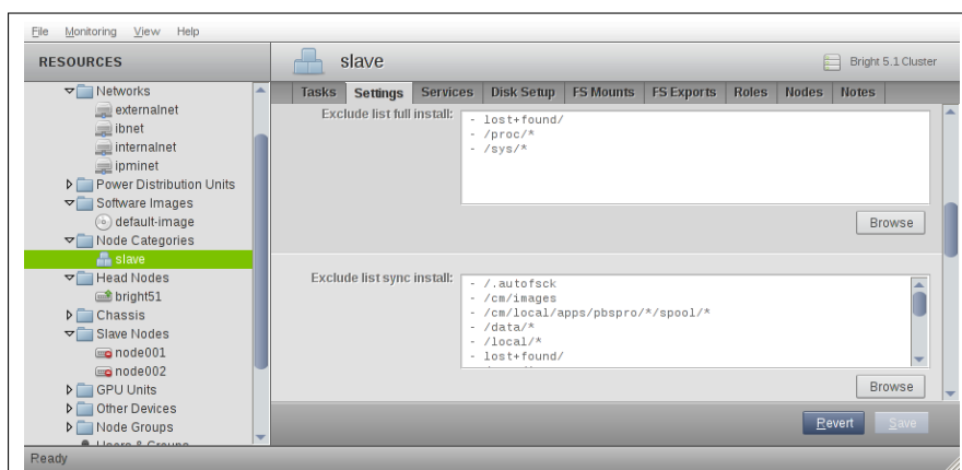
Figure 6.17: Setting up exclude lists with cmgui for provisioning
