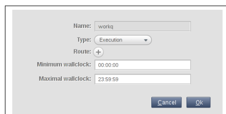
Figure 8.8: Workload Management Queues Edit Dialog For Torque And PBS Pro
