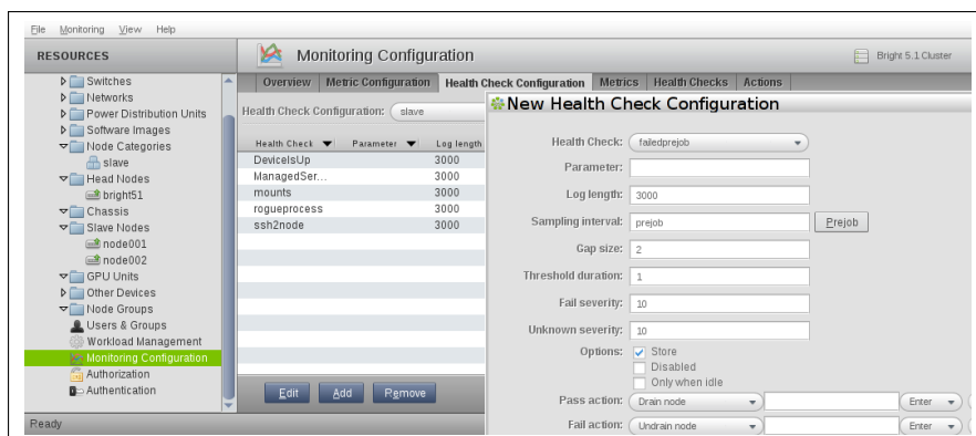
Figure 8.15: Configuring A Prejob Healthcheck Via cmgui
