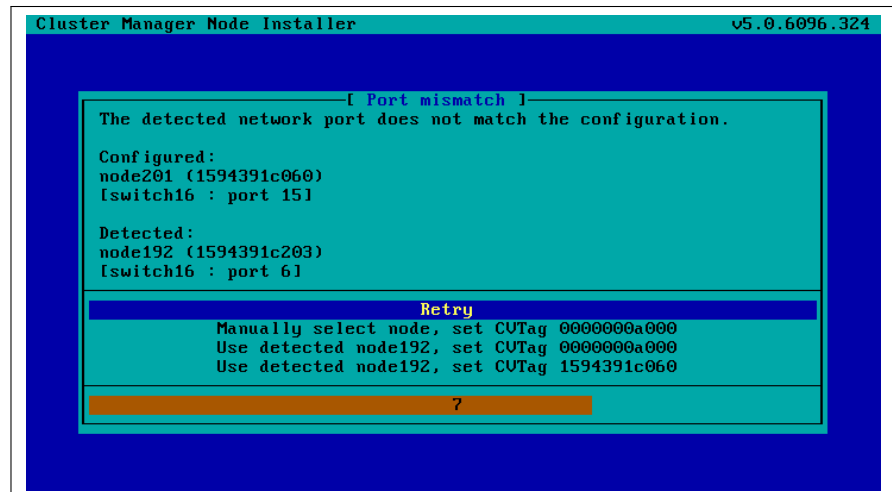
Figure 6.10: Scenarios: Port Mismatch Dialog
