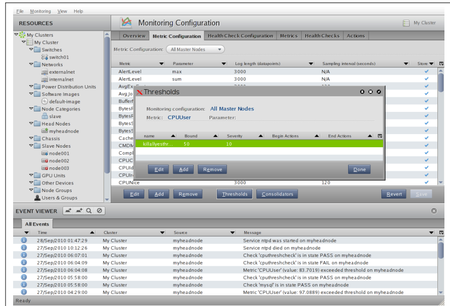
Figure 10.18: cmgui Monitoring: Thresholds Display
