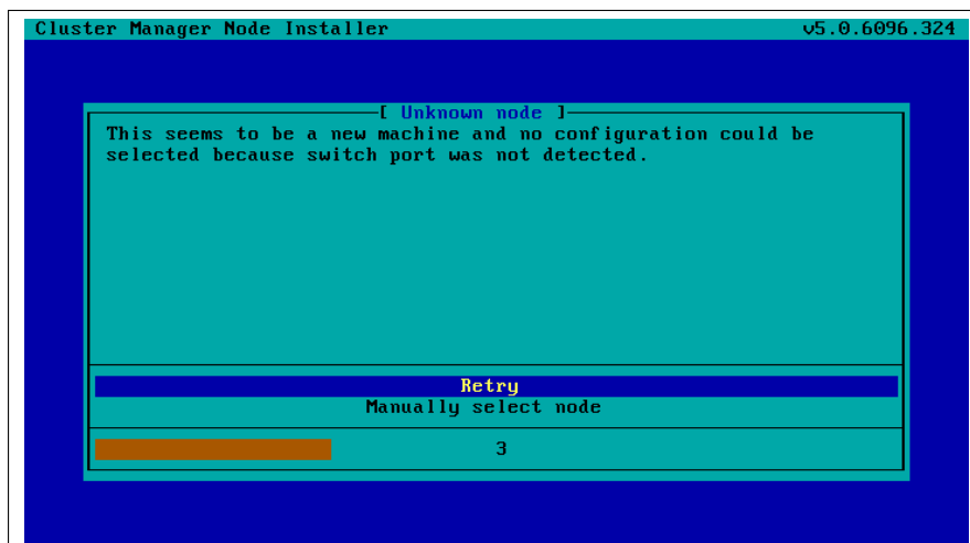
Figure 6.9: Scenarios: Unknown Node, No Ethernet Port Detected
