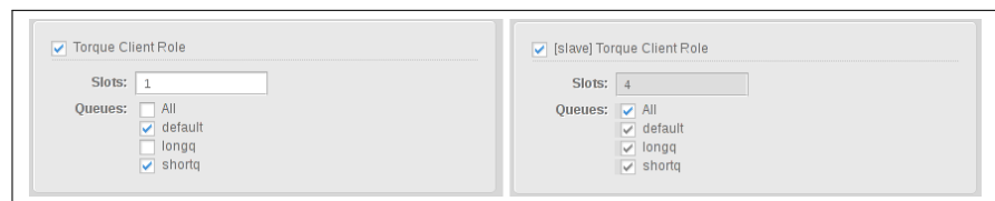
Figure 8.4: Workload Management Role Assignment Toggle States For An Individual Node
