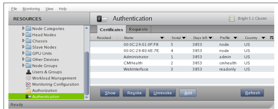
Figure 7.2: cmgui Certificates Tab
