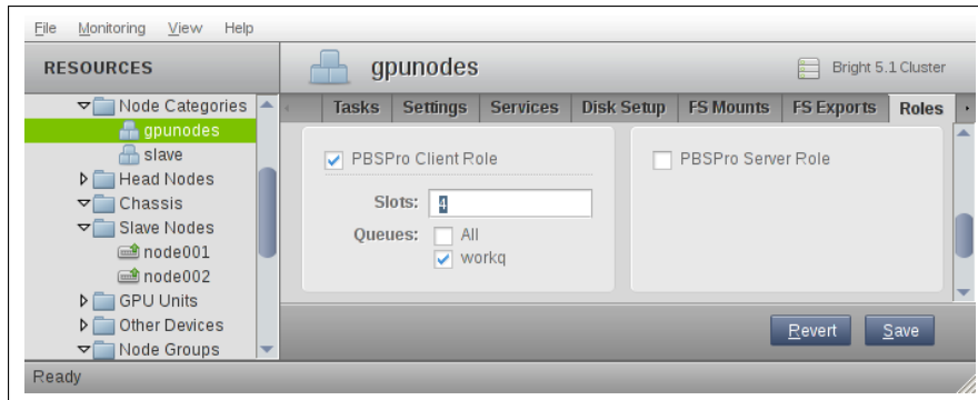
Figure 8.12: Setting A Queue For A New Category Via cmgui
