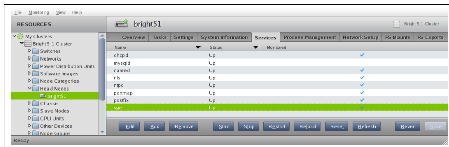
Figure 10.5: cmgui: Device Services Tab
