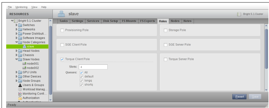
Figure 8.2: Workload Manager Role Assignment By Category For Compute Nodes
