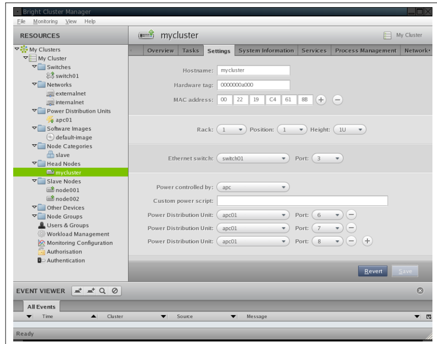
Figure 5.1: Head Node Settings
