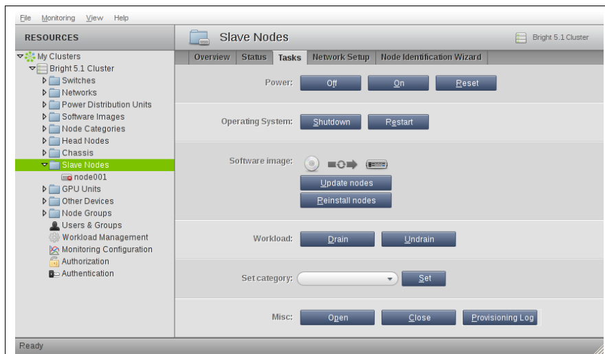
Figure 6.18: cmgui: Provisioning Log Button For A Device Resource
