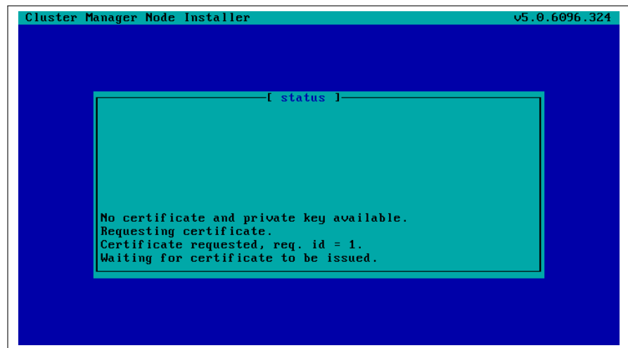
Figure 6.5: Certificate Request
