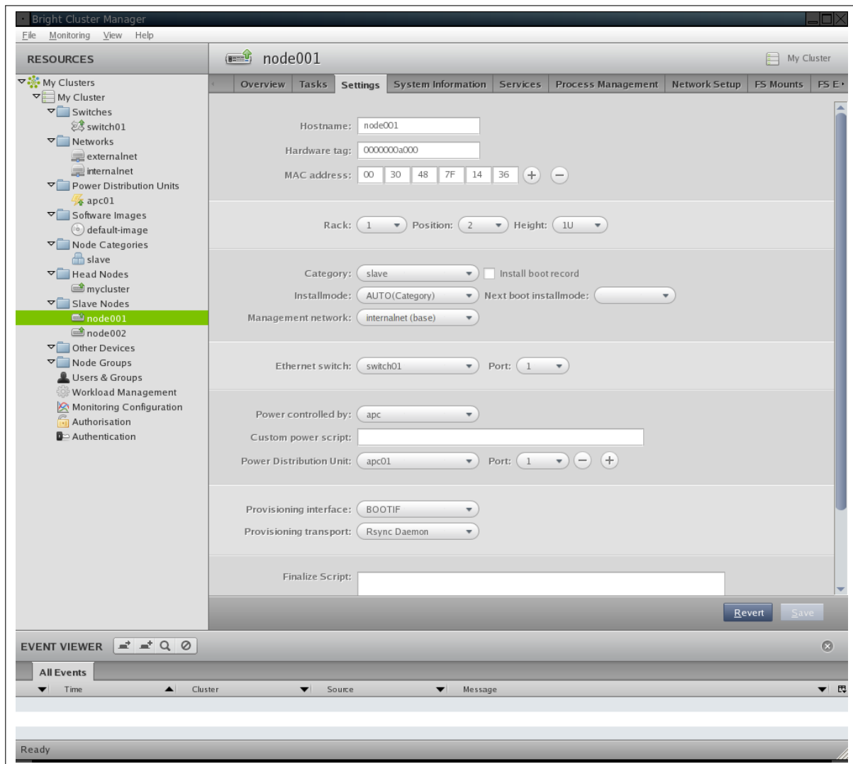
Figure 3.5: Node Settings
