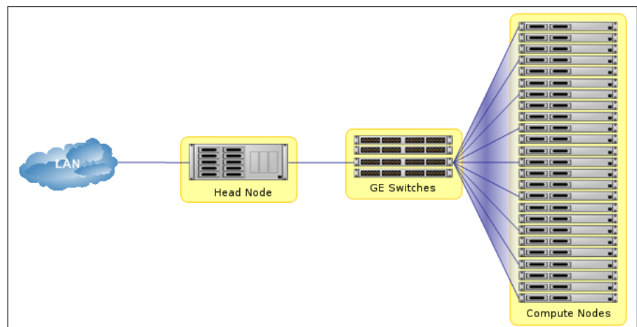
Figure 1.1: Cluster network
