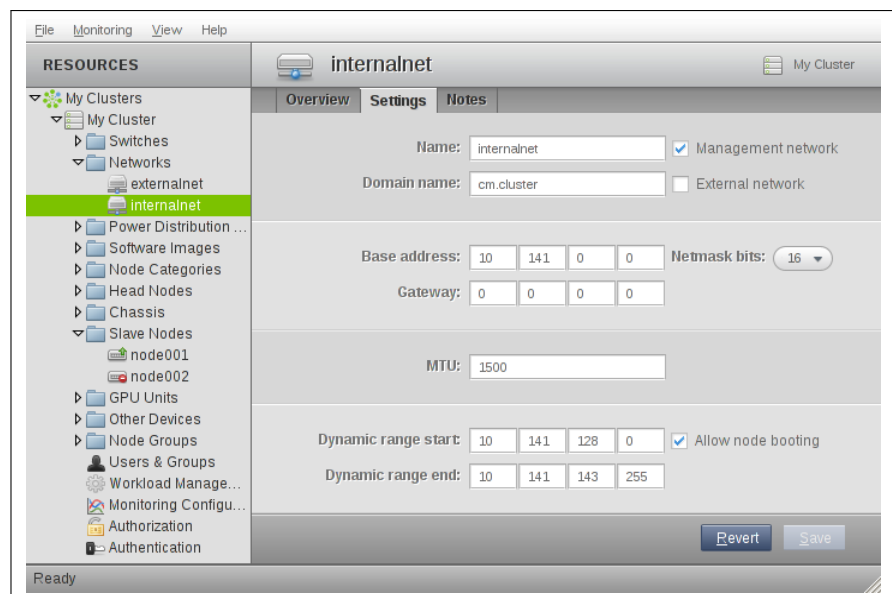
Figure 4.4: Network Settings
