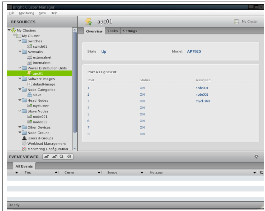
Figure 5.2: PDU Overview
