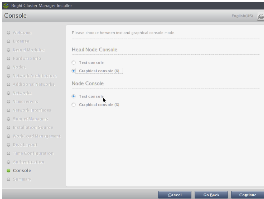
Figure 2.22: Console
