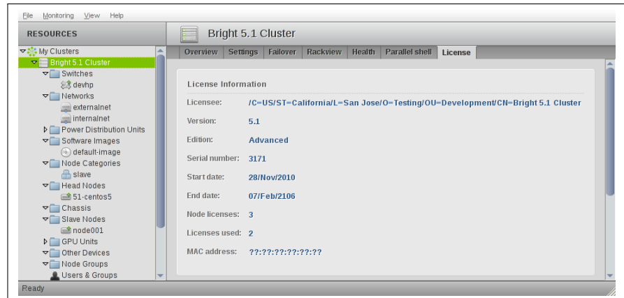
Figure 4.1: License Information
