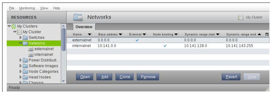
Figure 4.2: Networks
