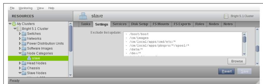
Figure 6.19: Setting up exclude lists with cmgui for node updates
