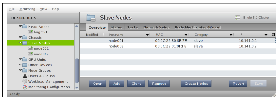
Figure 3.7: Nodes Overview
