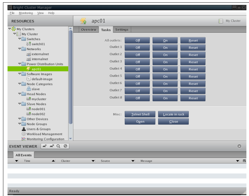
Figure 5.5: PDU Tasks
