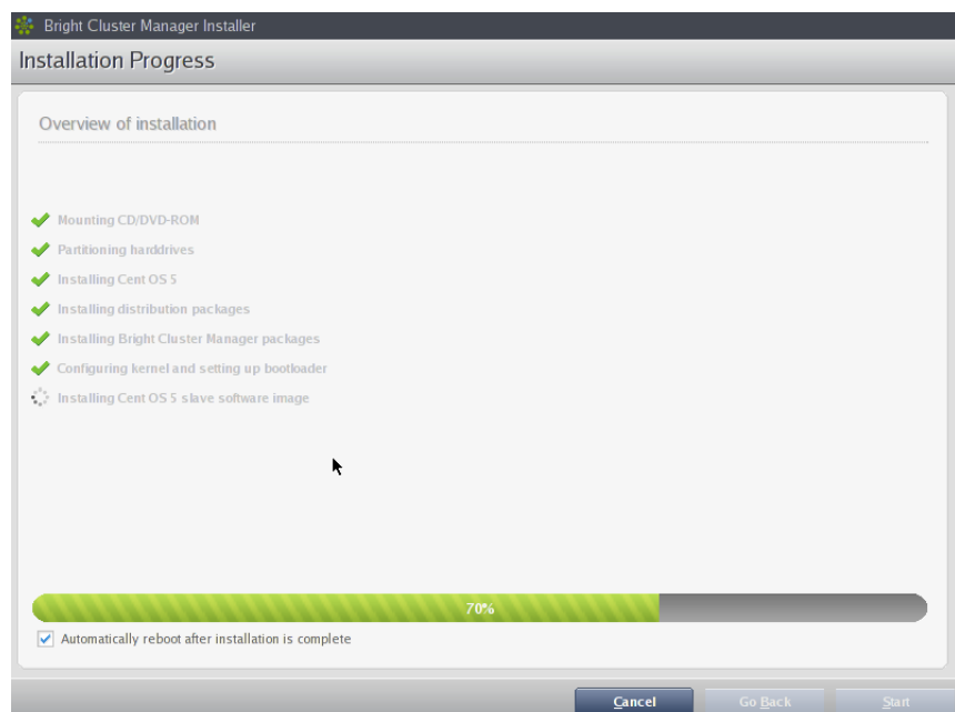
Figure 2.24: Installation Progress
