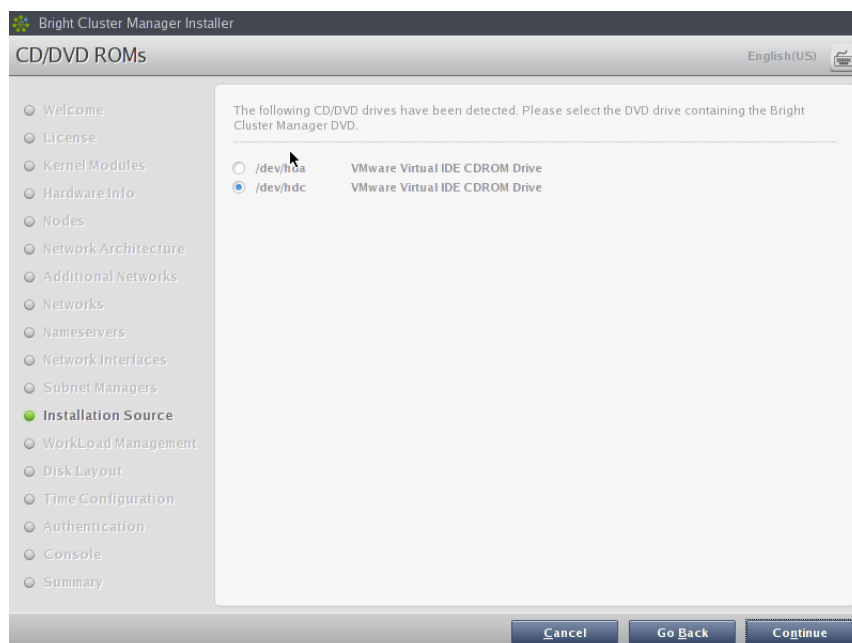
Figure 2.16: DVD Selection
