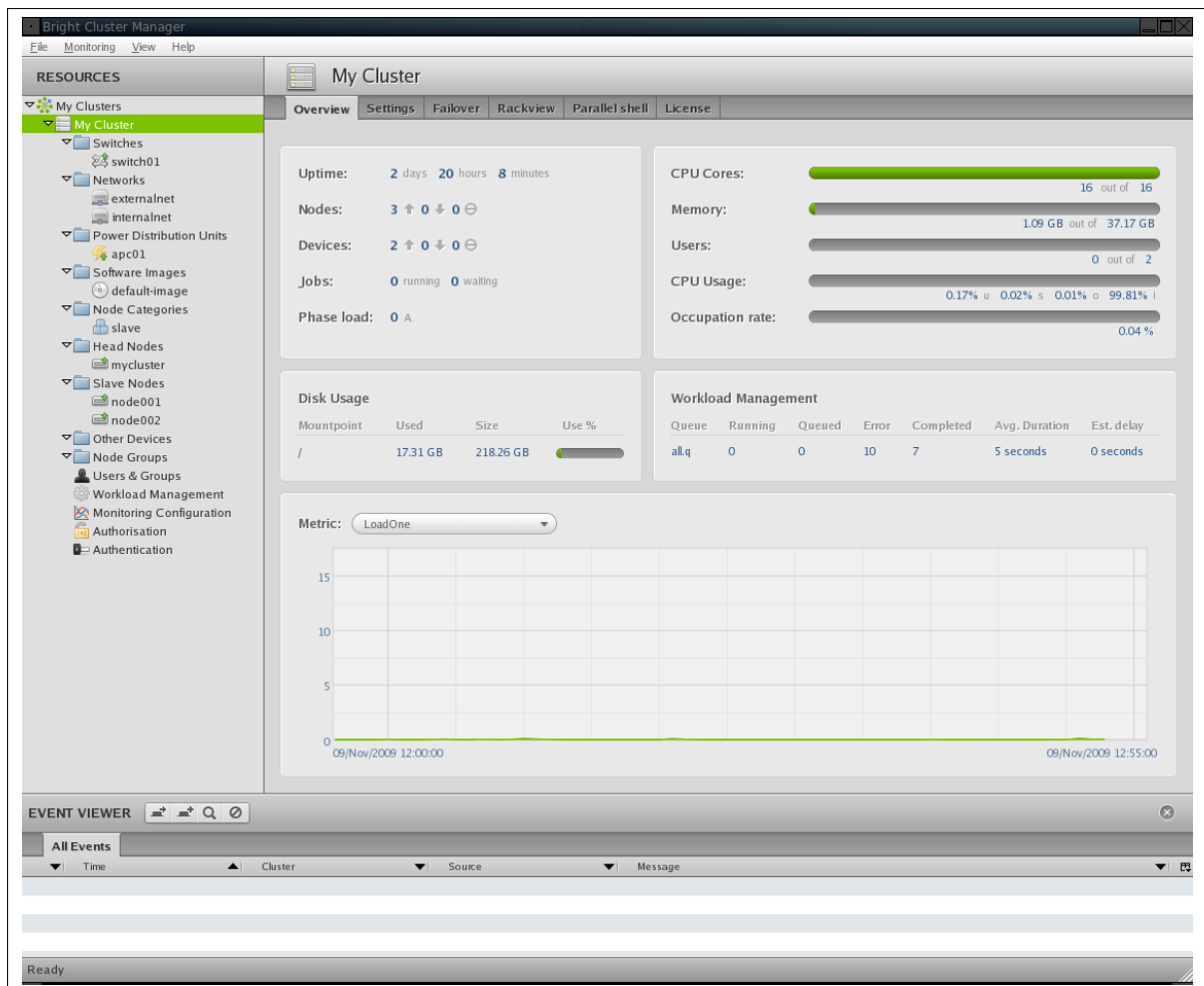
Figure 3.4: Cluster Overview
