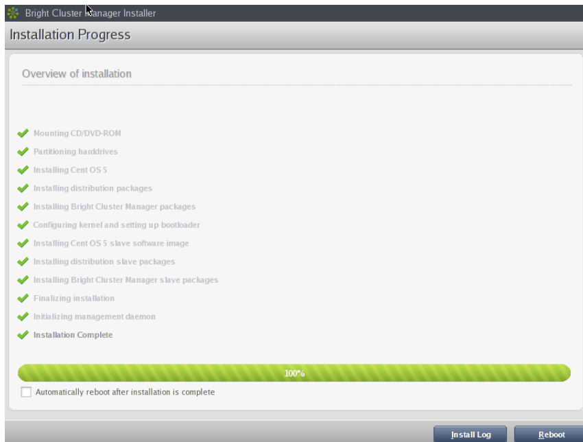
Figure 2.25: Installation Completed
