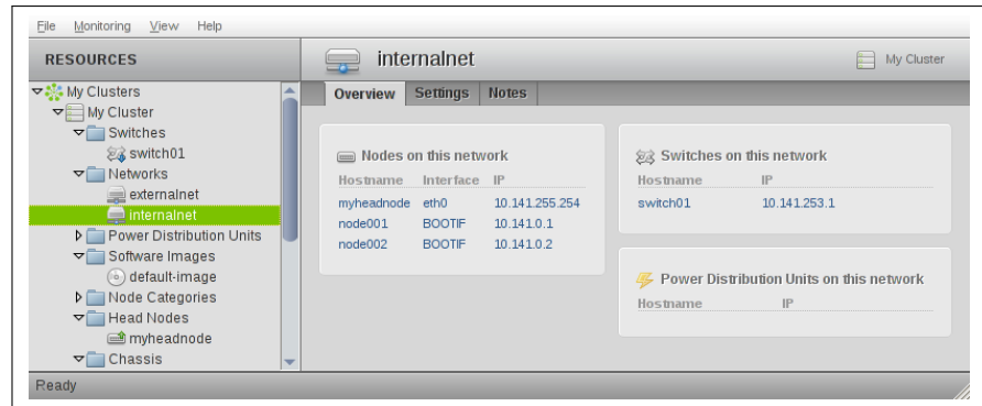
Figure 4.3: Network Overview
