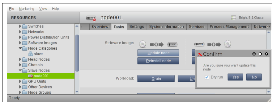
Figure 6.20: Updating A Running Node’s Image With cmgui
