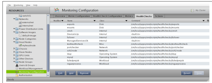
Figure 10.27: cmgui Monitoring: Main Health Checks Tab
