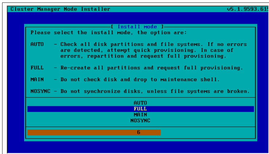
Figure 6.16: Install-Mode Setting Option During Node-Installer Run
