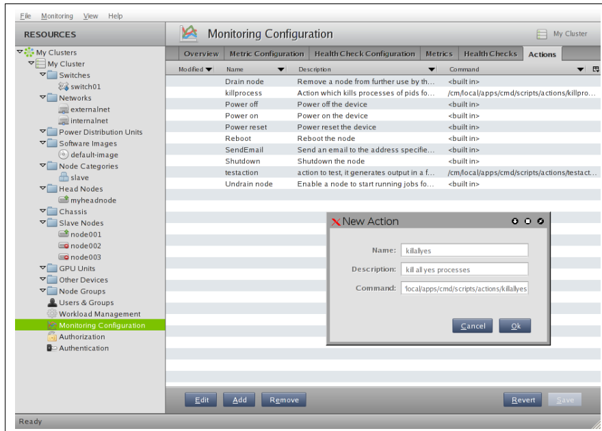
Figure 10.2: cmgui Monitoring Configuration: Adding An Action
