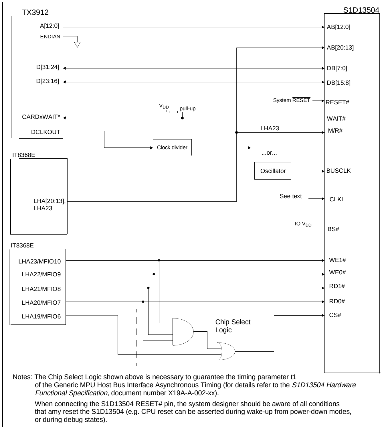
Figure 5-2: S1D13504 to TX3912 Connection using Two IT8368E
