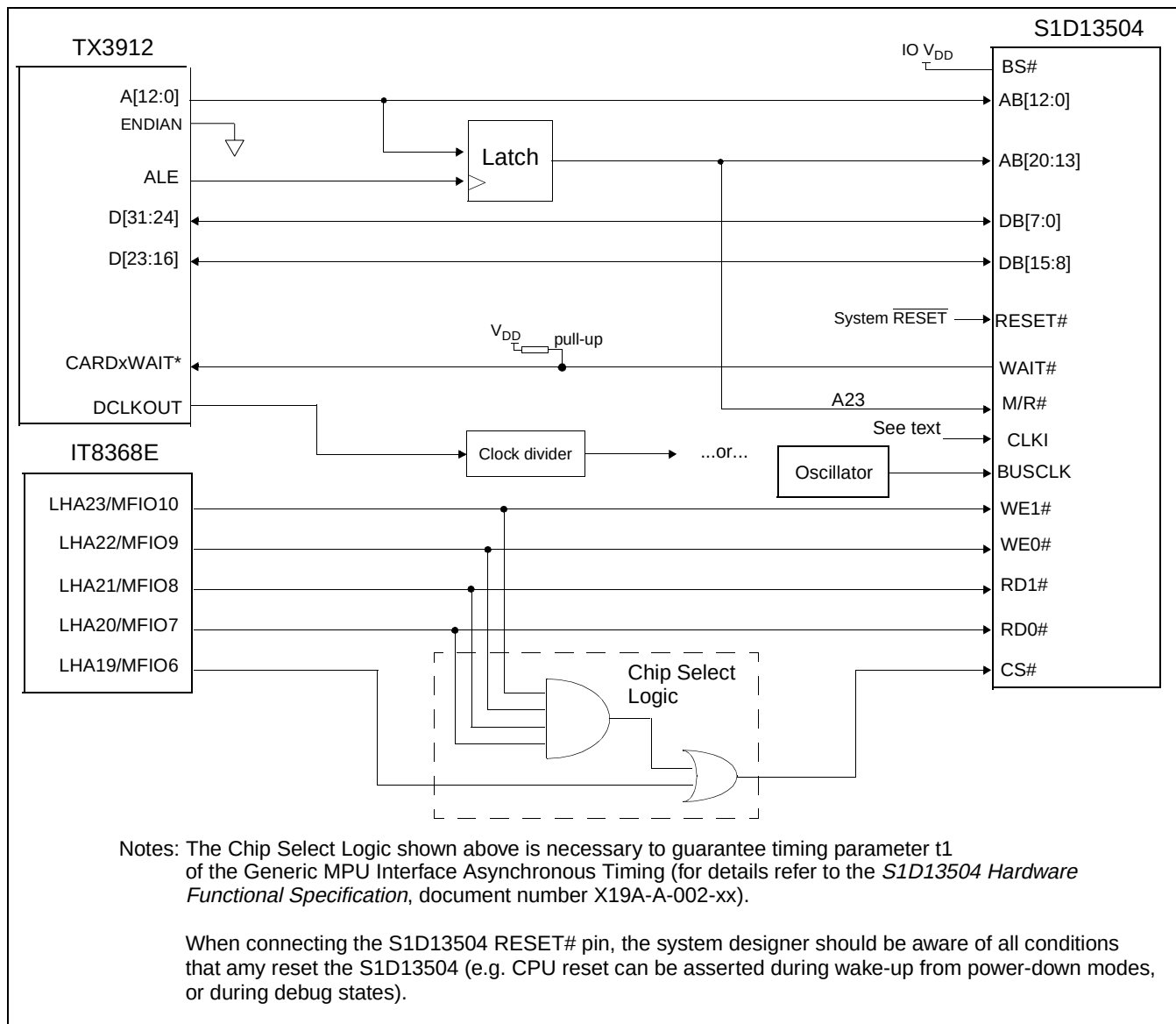
Figure 5-1: S1D13504 to TX3912 Connection using One IT8368E
