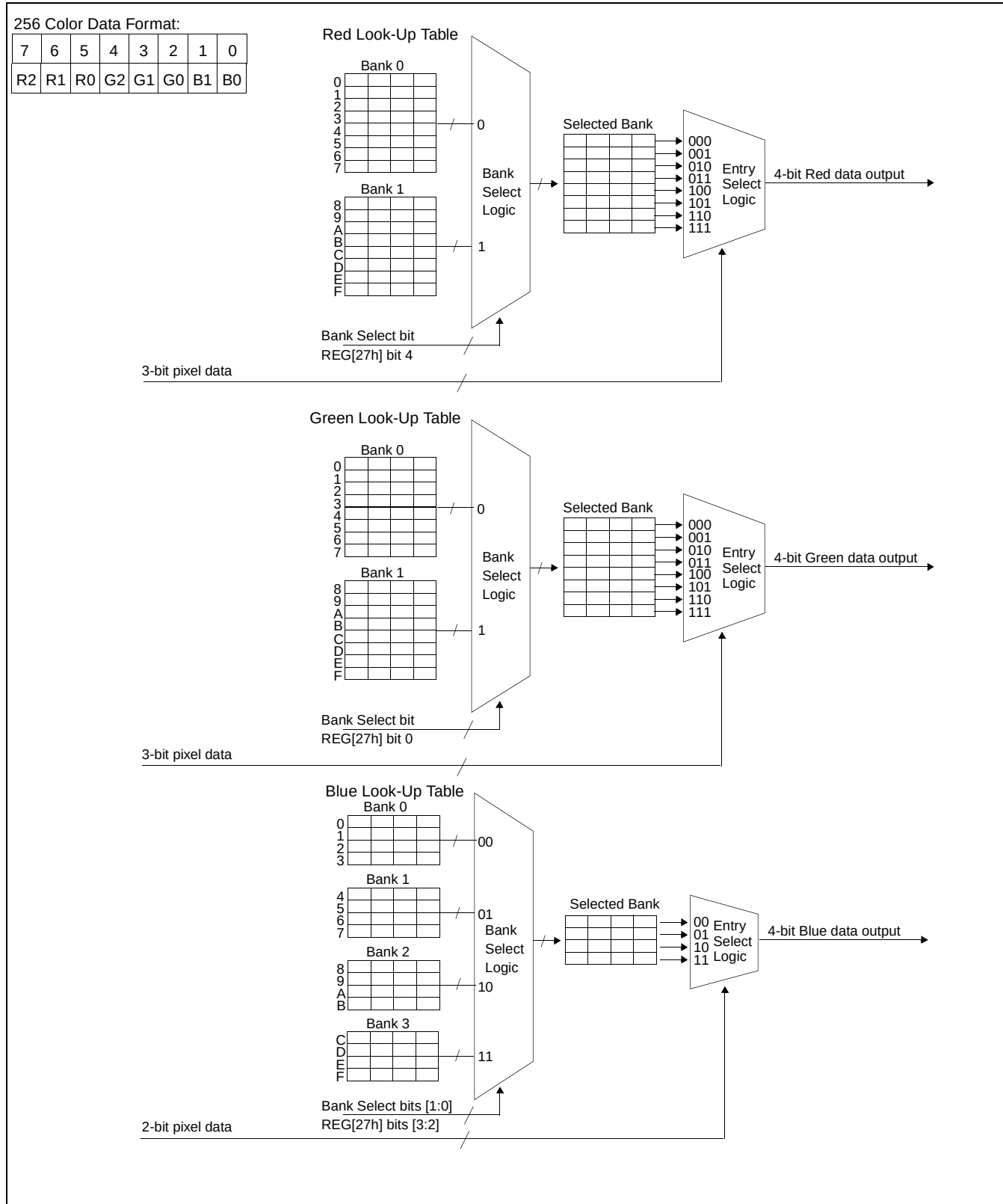
Figure 12-7: 8 Bit-Per-Pixel – 256-Level Color Mode Look-Up Table Architecture
