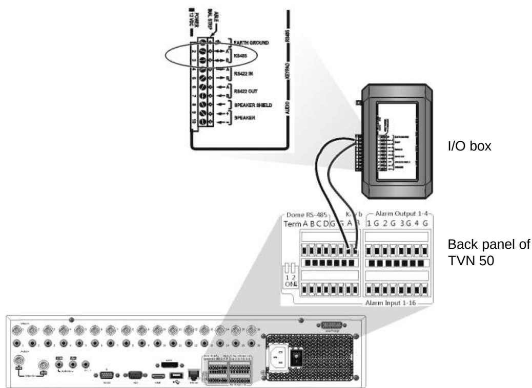
Figure 36: Keypad and NVR connections
