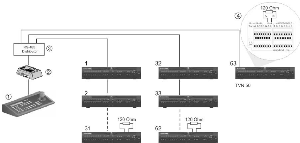
Figure 4: Expanding the system with an RS-485 signal distributor
