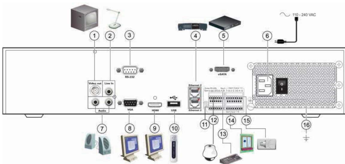
Figure 1: Back panel connections
