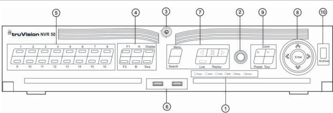
Figure 7: Front panel
