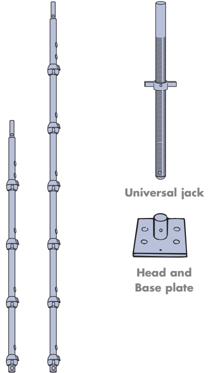
2m and 3m Standards
