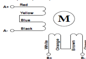
8-lead motor series connections
