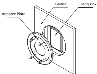
Figure 2-7 Secure the Camera Attachment
