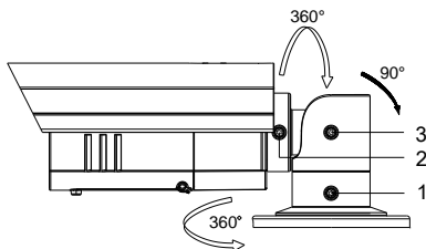
Figure 2-9 3-axis Adjustment
