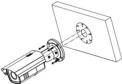
Figure 2-2 Secure the Camera
