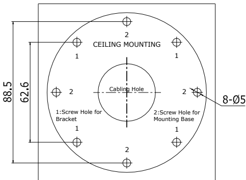
Figure 2-1 Drilling Holes in the Wall
