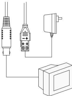
Figure 2-11 The Power and the Video Cable
