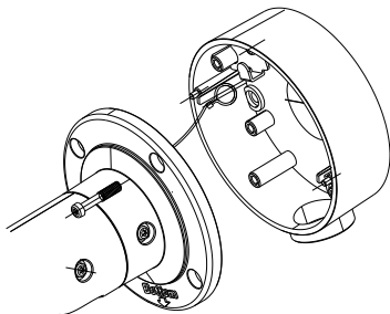
Figure 2-5 Hook the Camera to the Junction Box
