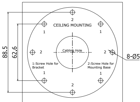
Figure 2-3 Drill Holes in the Wall
