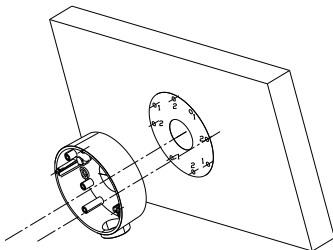
Figure 2-4 Secure the Junction Box
