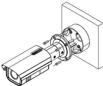
Figure 2-6 Secure the Camera
