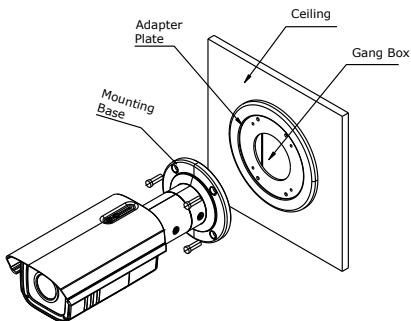
Figure 2-8 Secure the Camera
