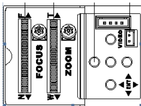
Figure 2-10 Zoom and Focus Adjustment
