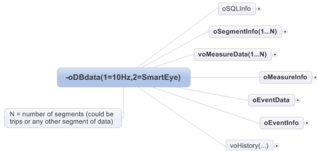
Figure 44: Overview of MATLAB struct oDBdata.mat.
