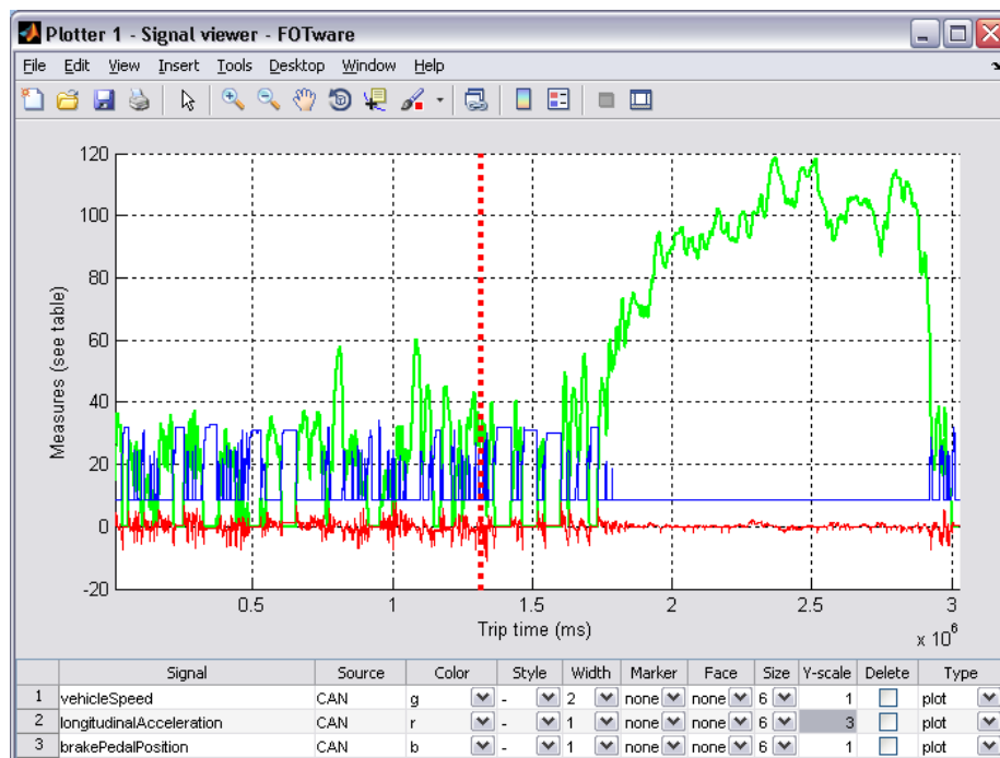
Figure 76: Three signals plotted in the signal plotter module.
