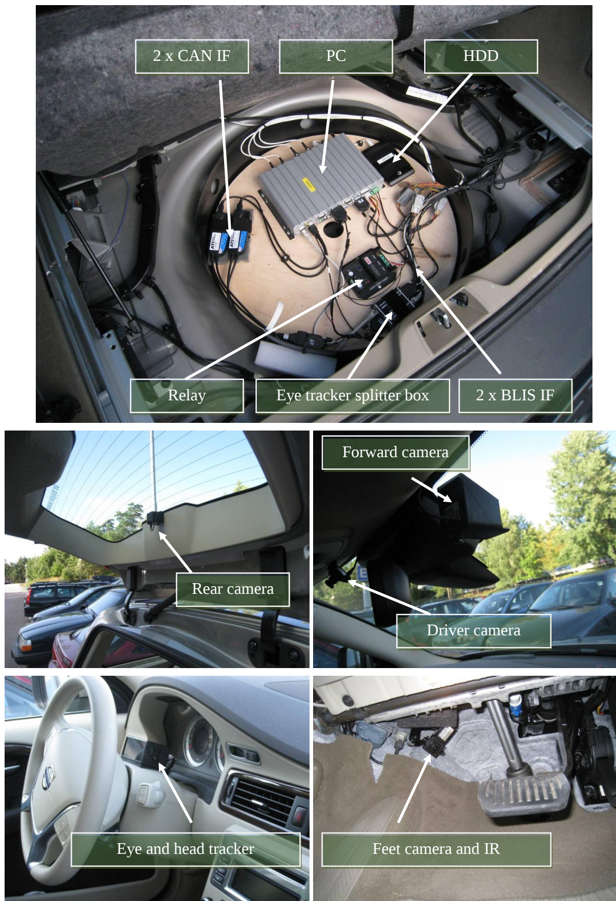
Figure 17: Swedish VMC - Placement of DAS including extra sensor and cameras.
