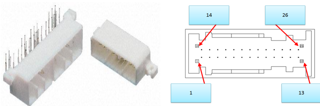
Figure 8: Tyco Connector.
