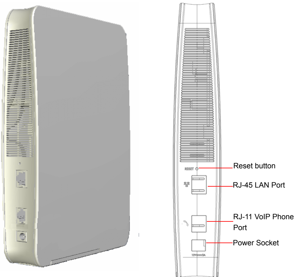
Figure 2-2: BreezeMAX Si 4000 Rear Panel
