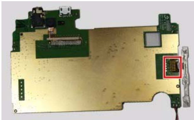
Figure 7-15. Position of desoldering the side key FPC
