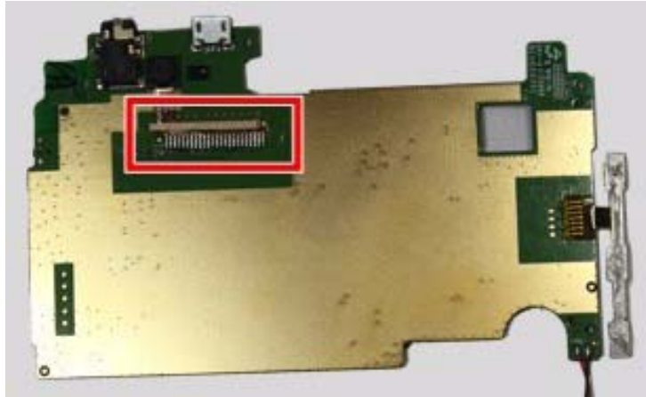
Figure 7-18. Position of desoldering the FPC of the front camera
