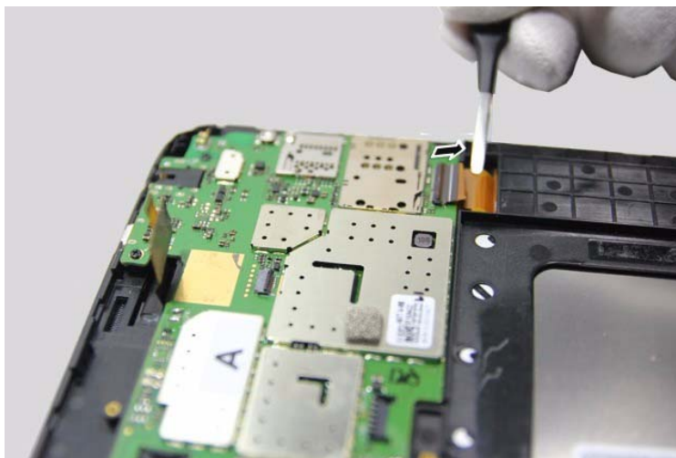
Figure 7-11. Pulling out the LCD FPC
