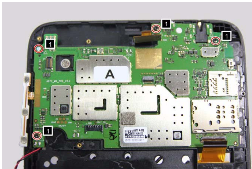
Figure 7-12. The screws for fixing the PCBA
