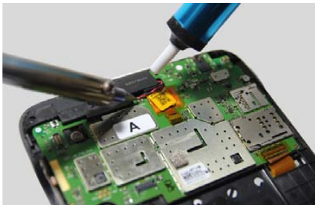
Figure 6-1. Desoldering the receiver wires
