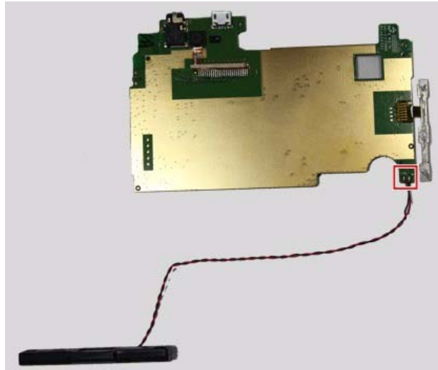
Figure 7-16. Position of desoldering the speaker wires
