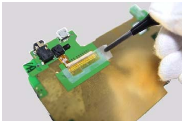
Figure 7-17. Peeling off the conductive fabric and mylar
