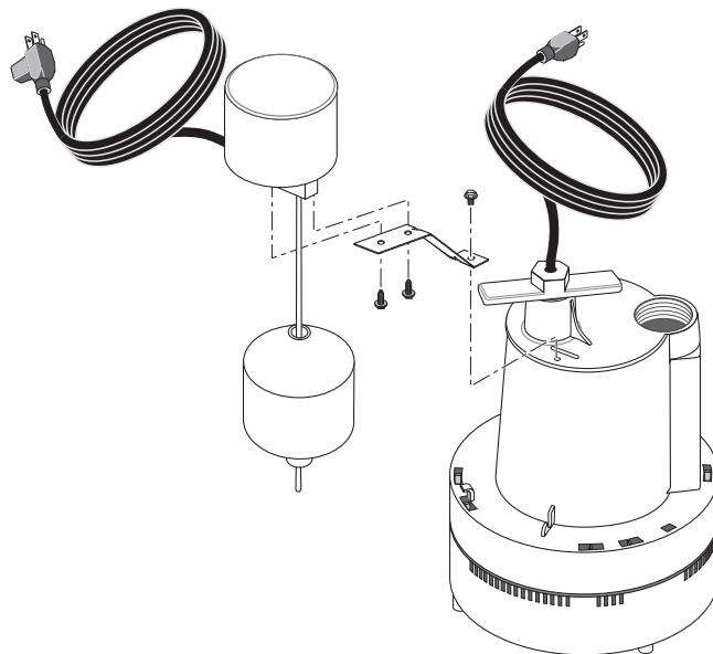
Figure 2: Vertical Float Switch Replacement.
