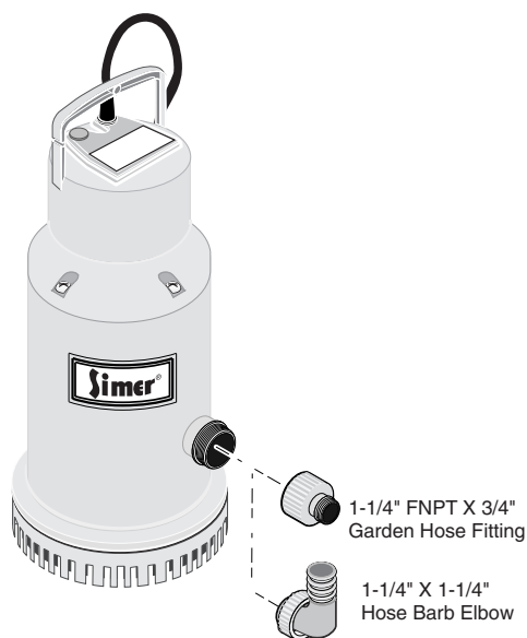
Figure 2: Adapter connections.
