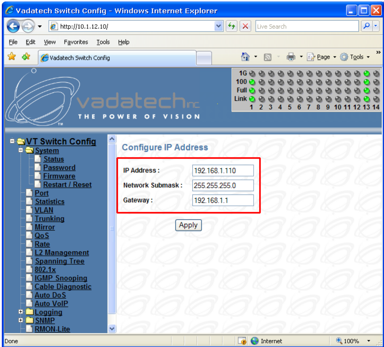
Figure 2: Gigabit Ethernet Switch IP address configuration
