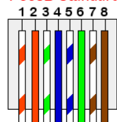
T-568B Standard
