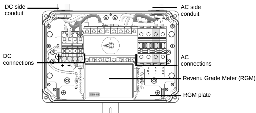
Safety Switch for single phase inverter 10-11.4kW with built-in RGM
