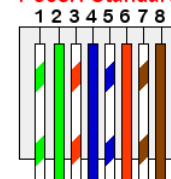
T-568A Standard
