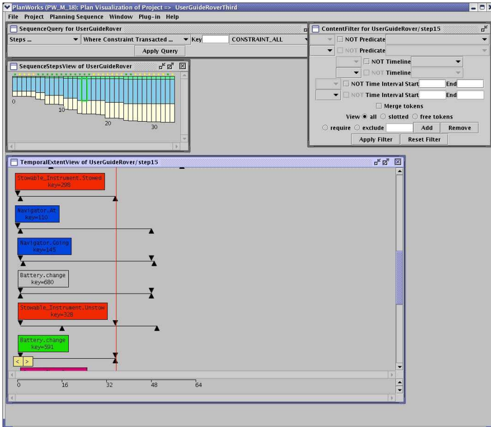
Figure 12: EUROPA 2 PlanWorks Temporal Extent View
