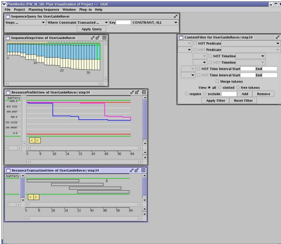
Figure 10: EUROPA 2 PlanWorks Resource Profile and Transaction View
