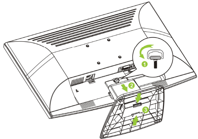
Figure.1. Installing and Removing the Base
