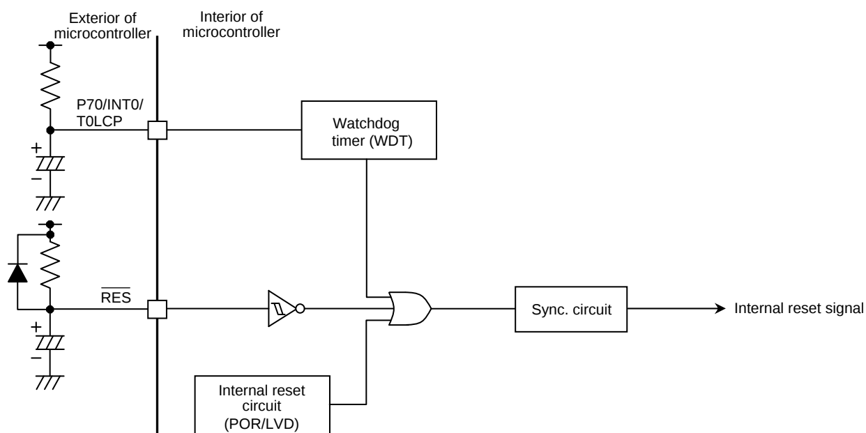
Figure 4.4.1 Sample Reset Circuit Block Diagram
