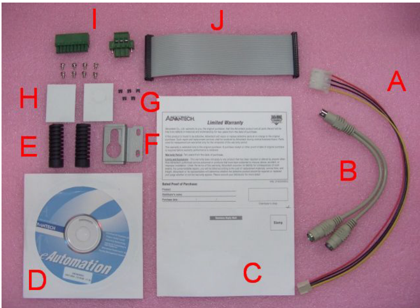
Figure 1.3: UNO-3072L Accessories
