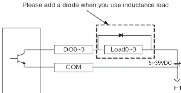
Figure 2.7: Isolated Digital Output Connection
