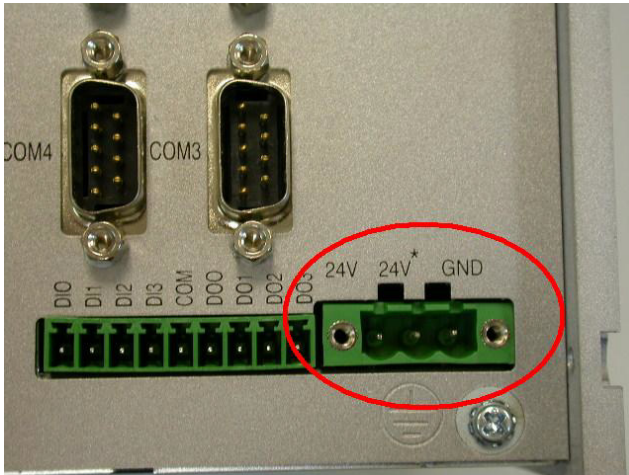
Figure 2.11: Location of Power P1 and P2
