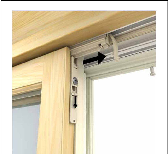
Depress the sash retainer bar latch and slide the retainer bar away from the sash.
