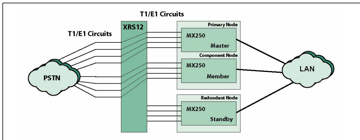
Figure 16-5 MX Cluster Topology – 2:1 Redundancy in Normal Mode
