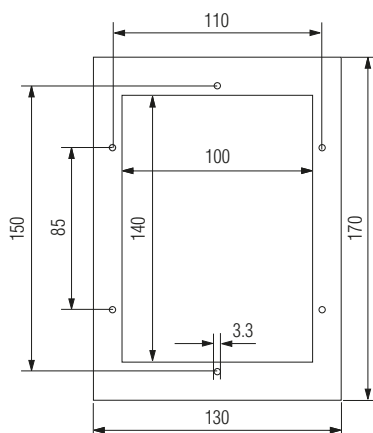
Dimensions and wall cut-out (mm)
