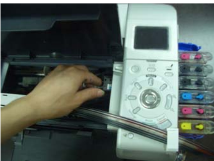
Adjust the tube length and move the cartridge carriage to the leftmost and rightmost. Make sure that there will be no block and collision when the cartridge moves.
