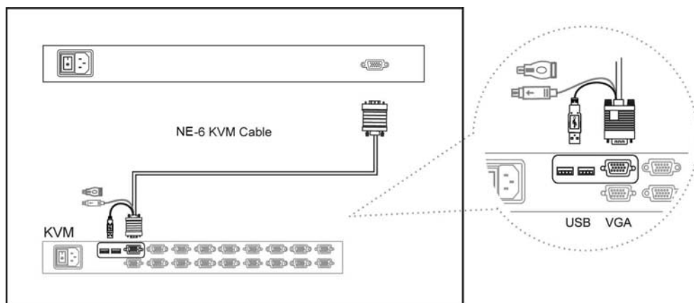
Figure12. Example of connecting NE-6 4-in-1 Combo KVM cable to KVM via USB interface
