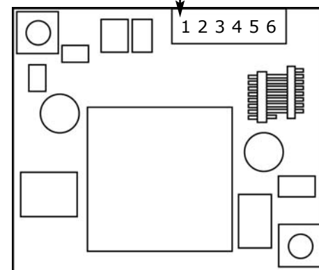
20K15X (6 Pin) Backside J2 pad connector
