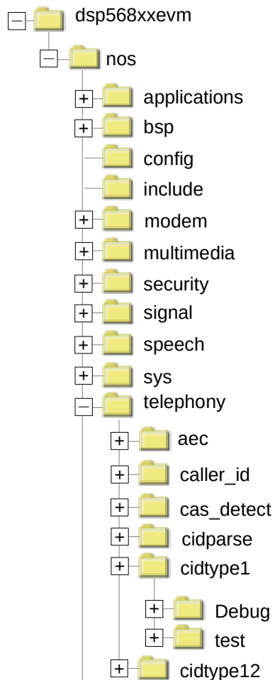
Figure 2-2. cidtype1 Directory
